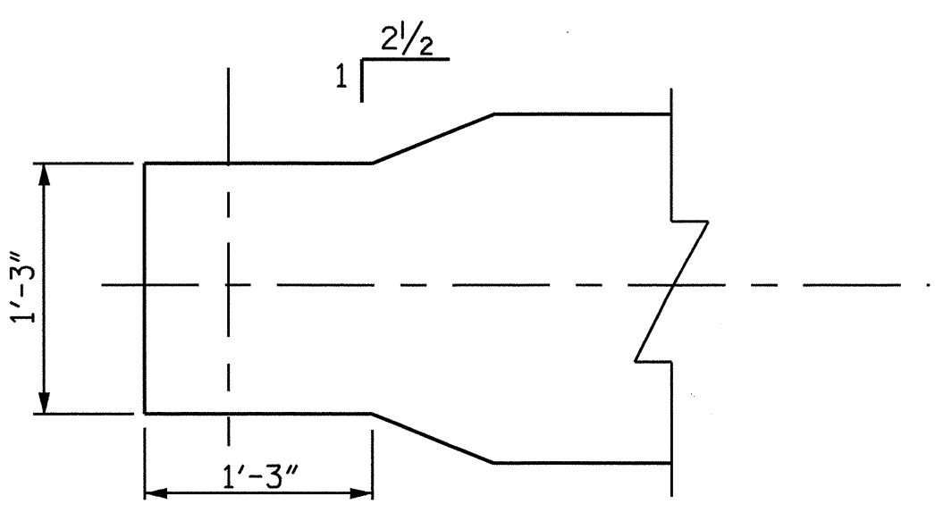
BOTTOM FLANGE DETAIL @ END BENTS
