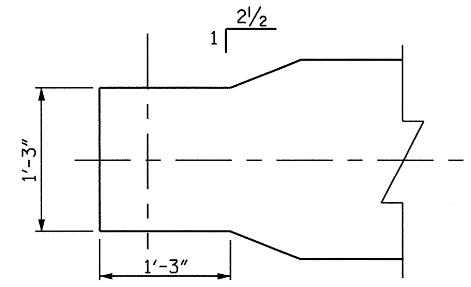
BOTTOM FLANGE DETAIL @ END BENTS
