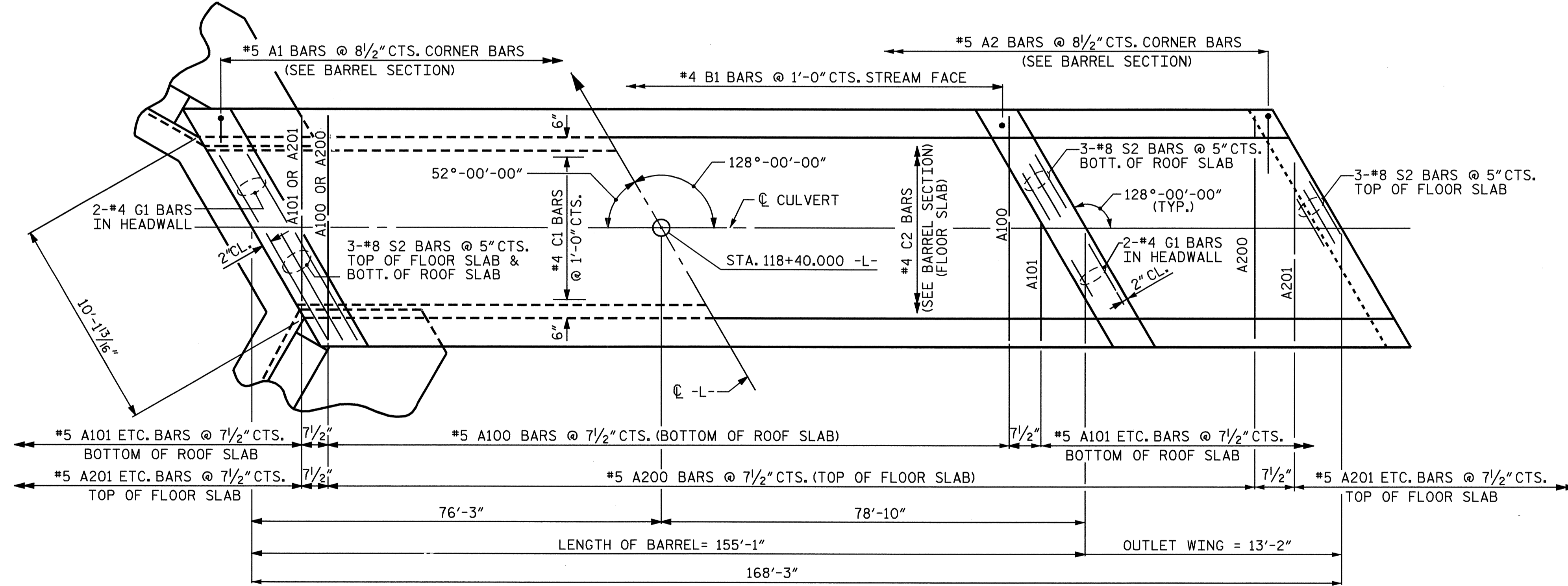
PLAN OF CULVERT
