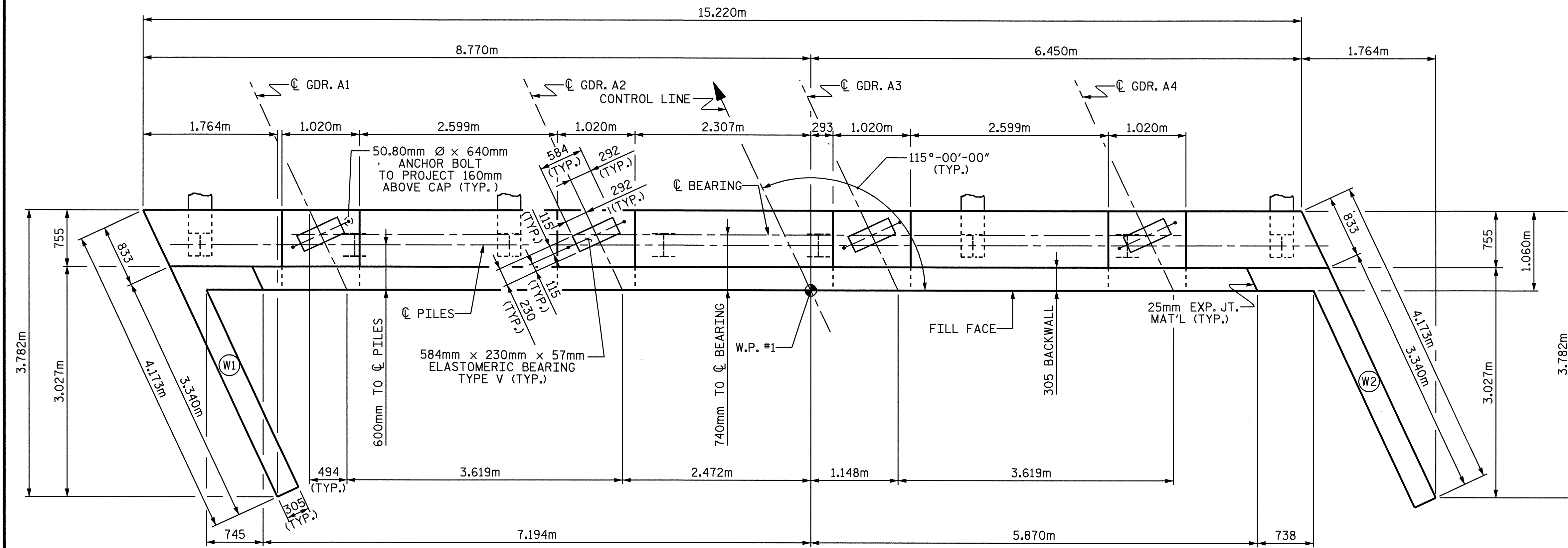
PLAN
