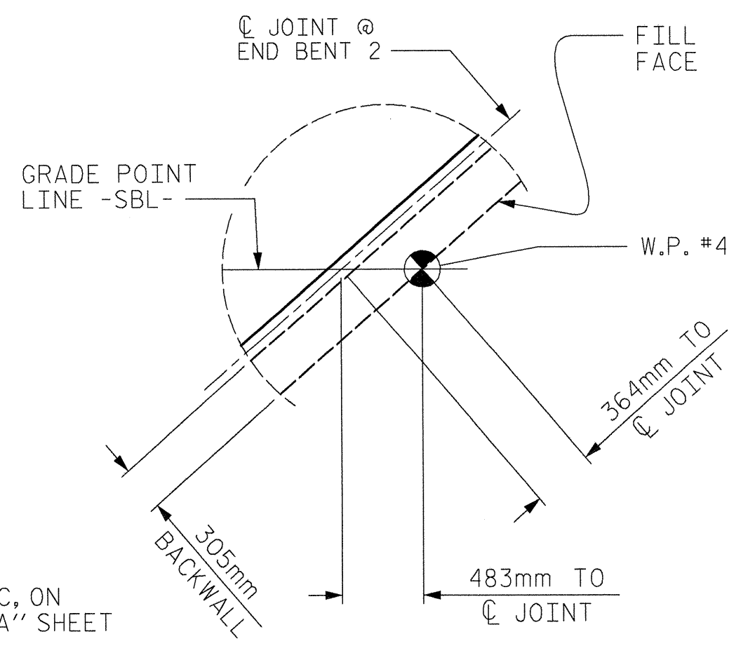
DETAIL D
