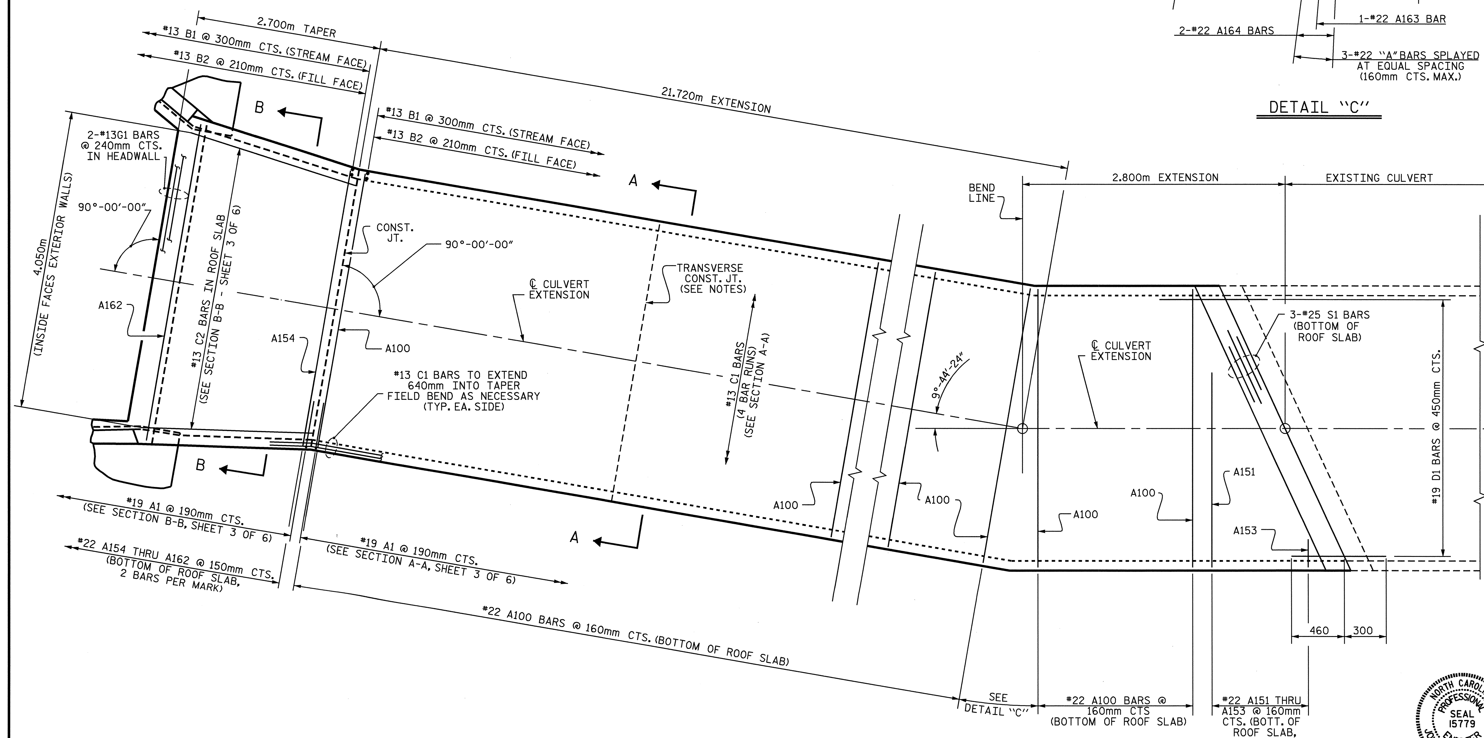
PLAN - ROOF SLAB
