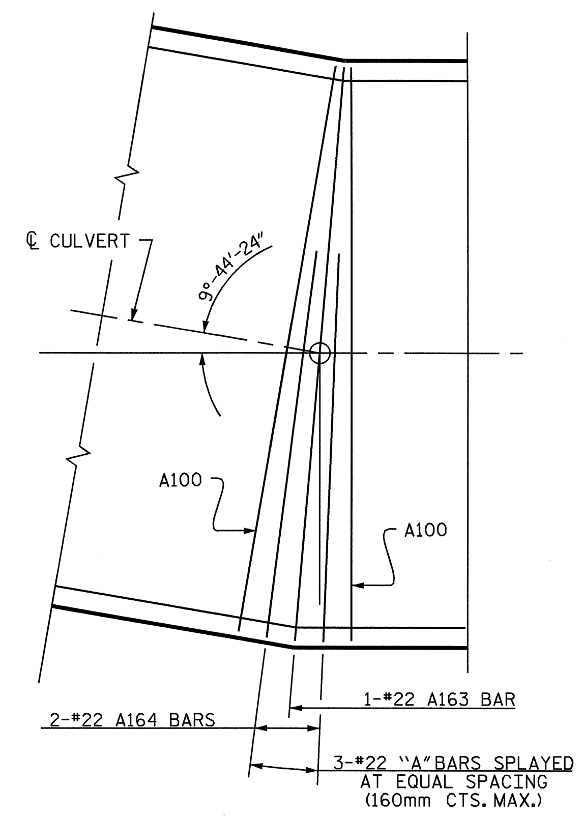
DETAIL "C"
