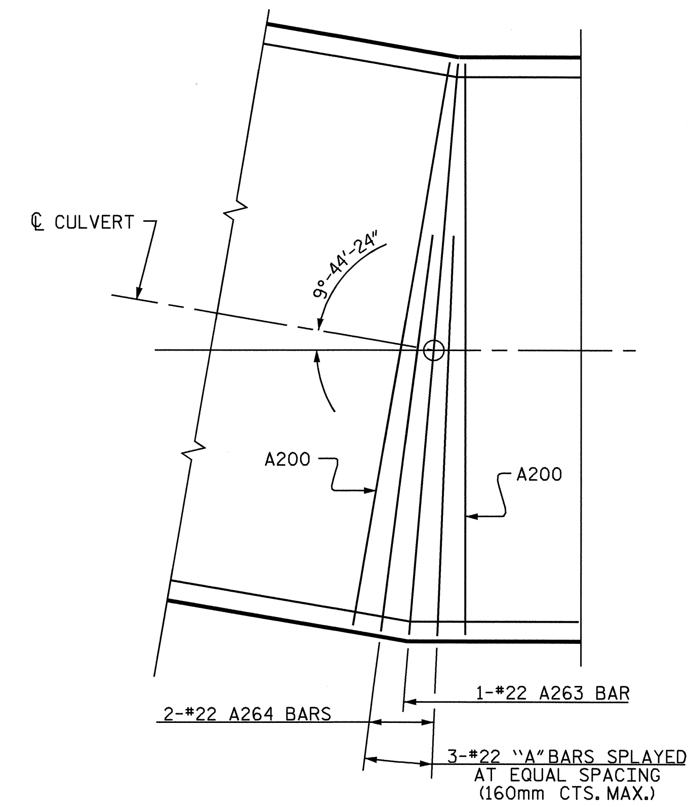
DETAIL "D"
