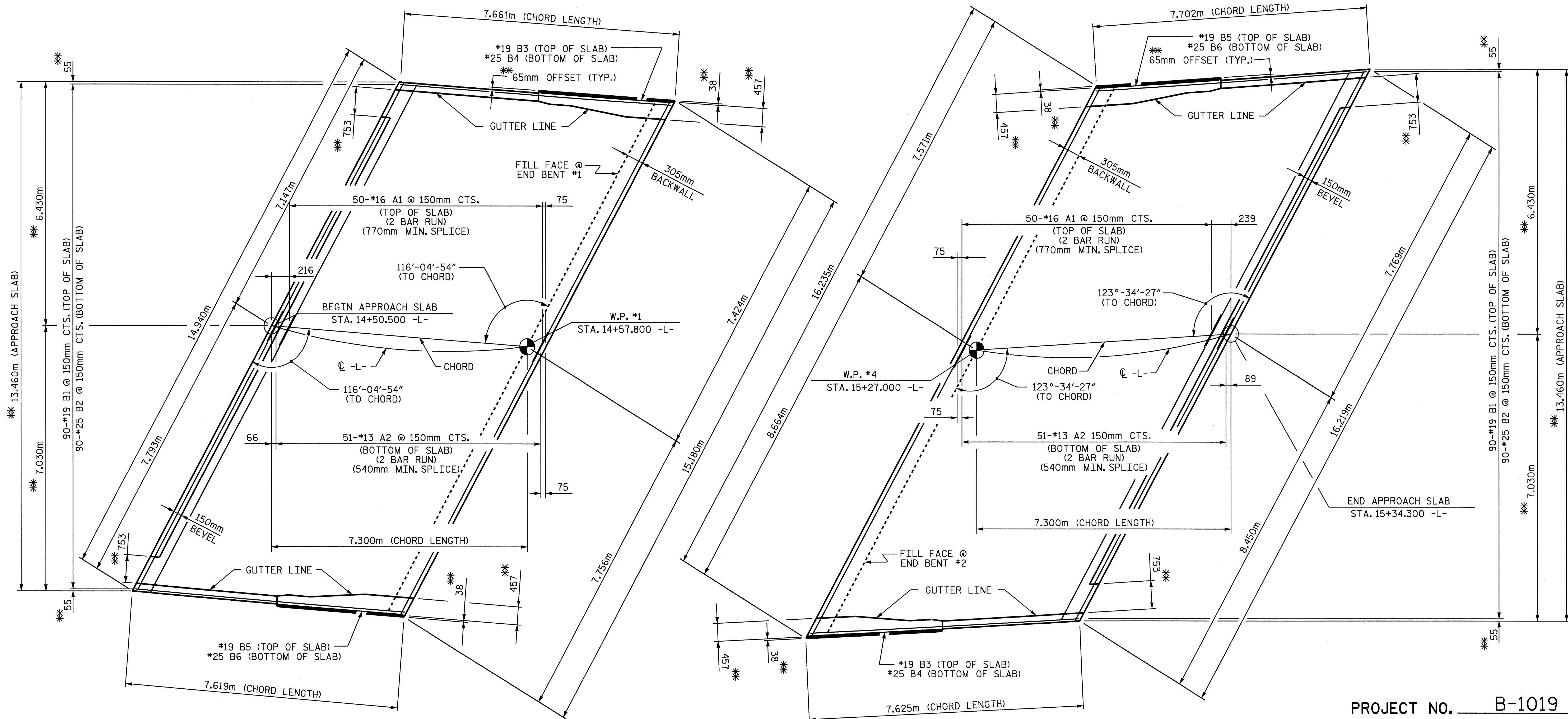
PLAN OF APPROACH SLAB AT END BENT #1
