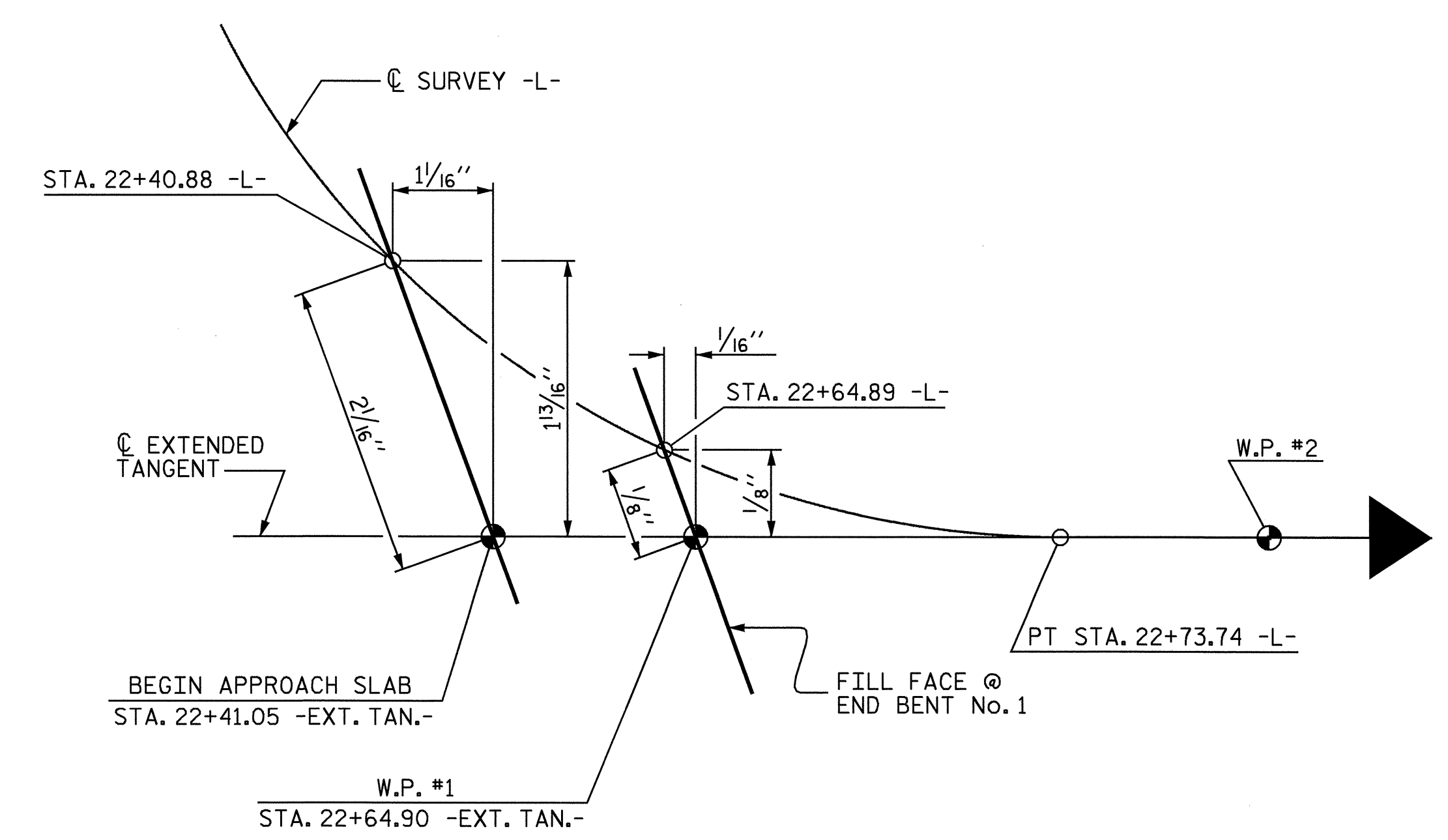
EXTENDED TANGENT LAYOUT
