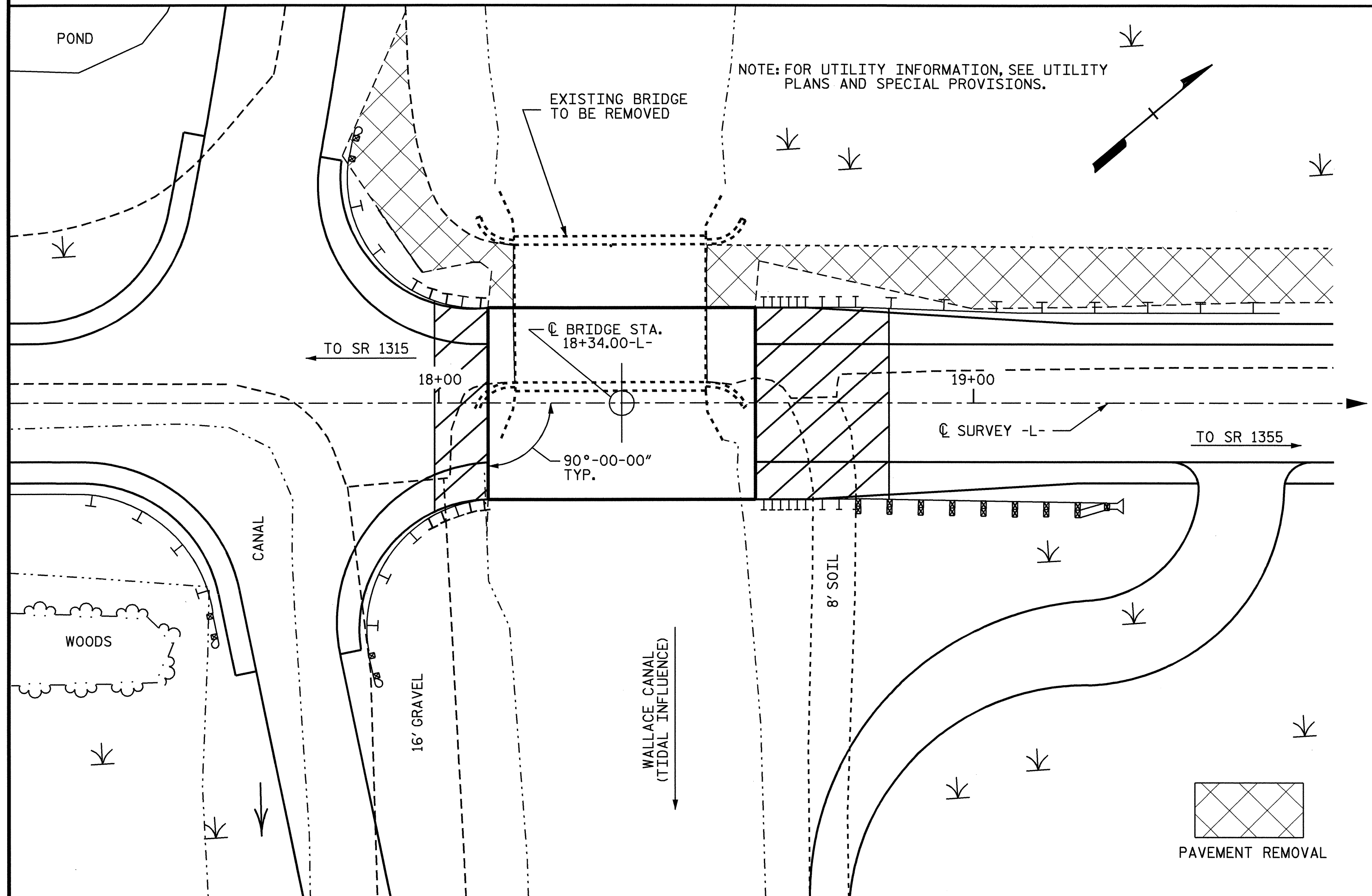
LOCATION SKETCH
