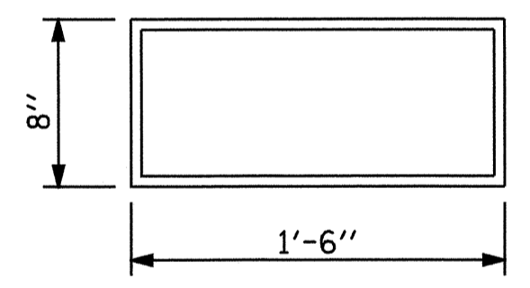
E1 (24 REQ'D) PLAN VIEW OF ELASTOMERIC BEARING TYPE III
