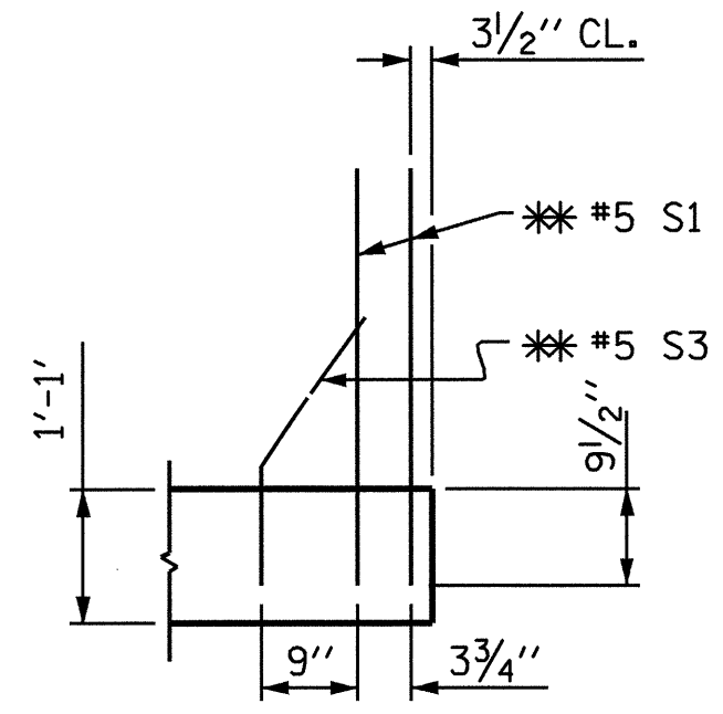
SECTION K-K ** ADHESIVELY ANCHORED
