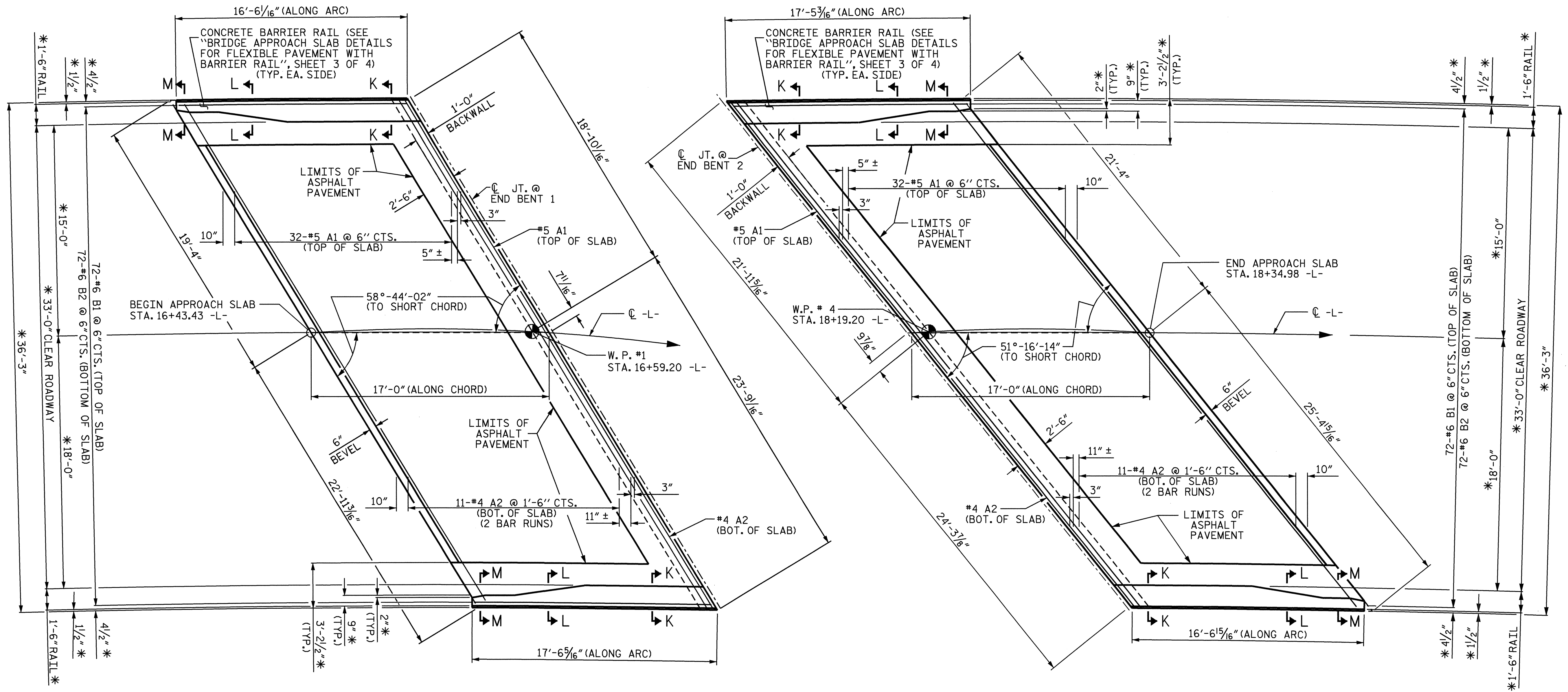
@ END BENT 1
