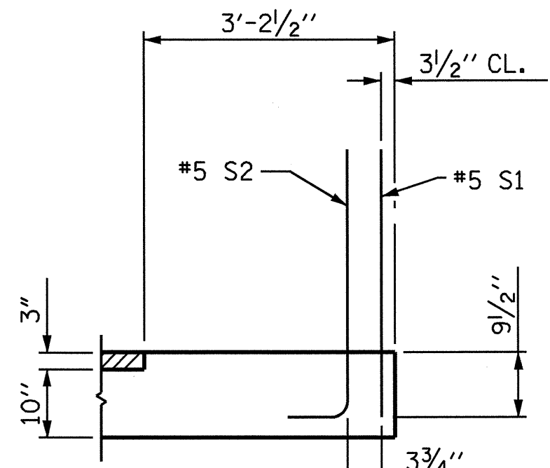
SECTION M-M
