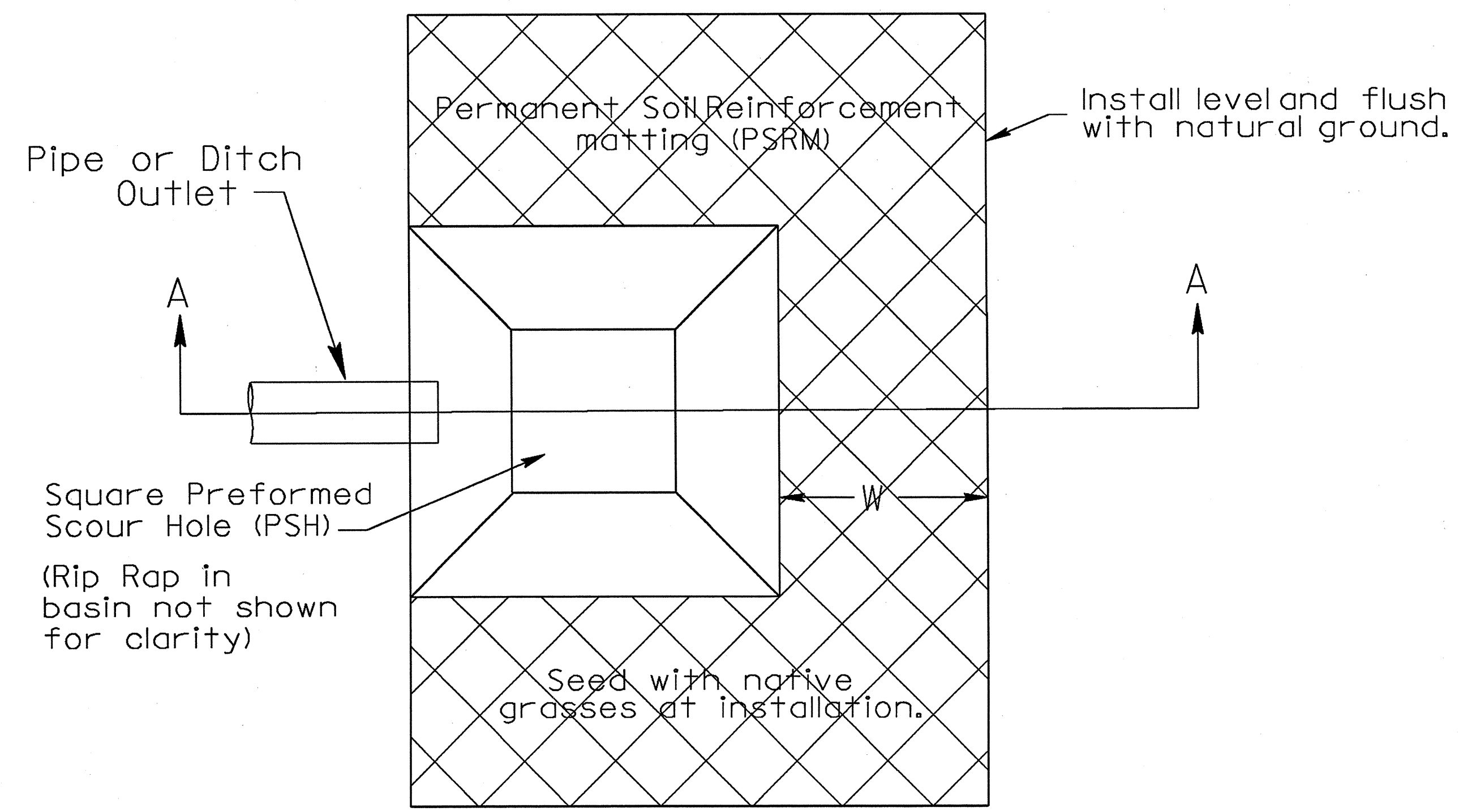
PLAN VIEW
