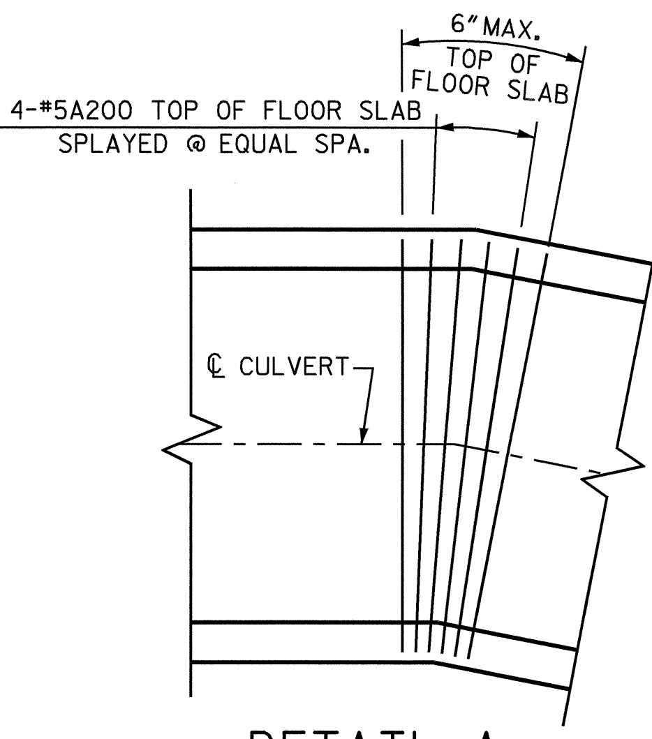
DETAIL A
