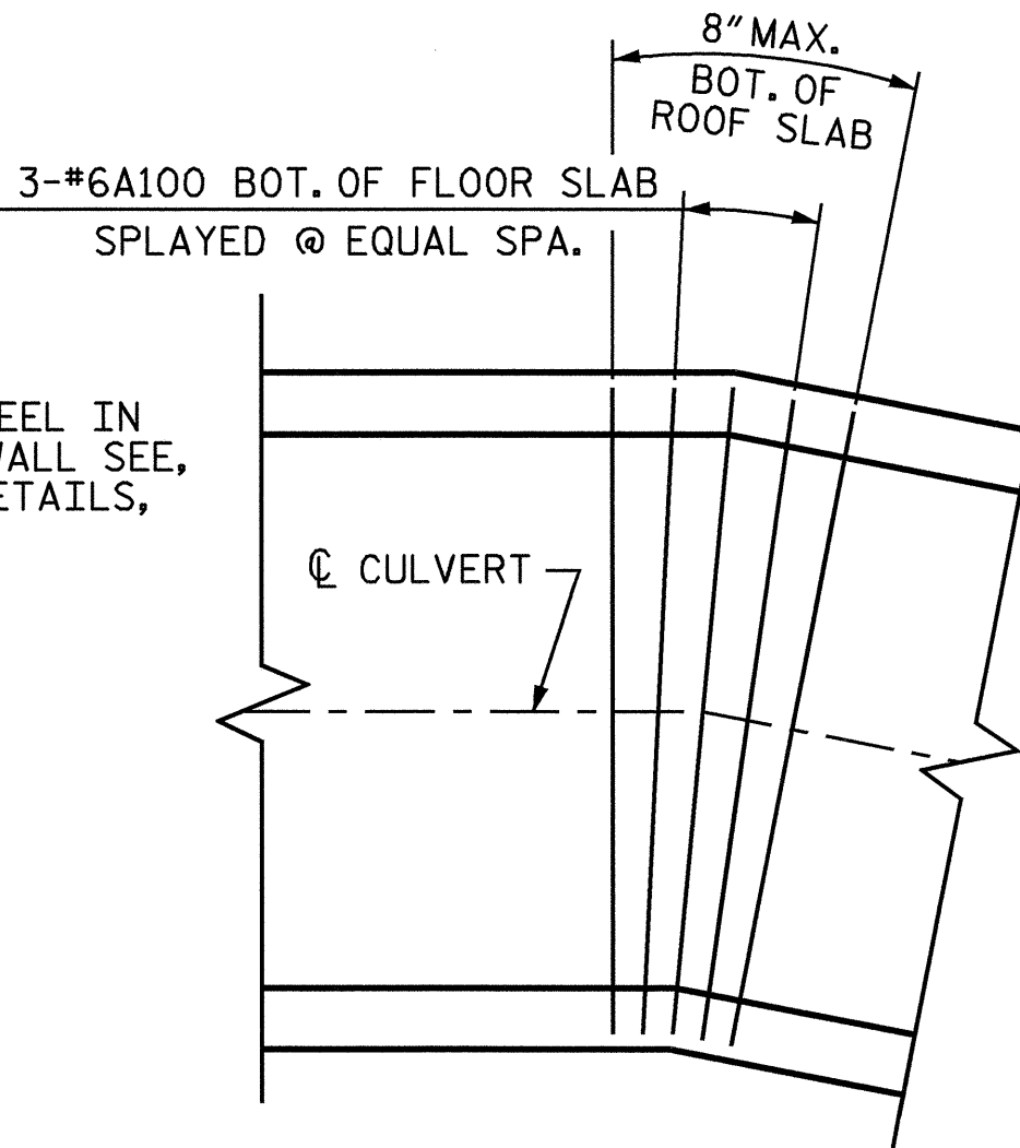
DETAIL B
