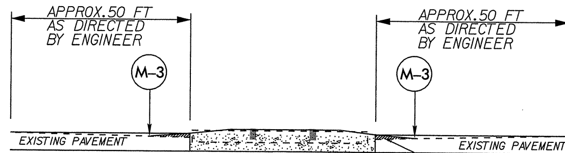
DETAIL NO. 3 MILLING RAILROAD CROSSING APPROACH
