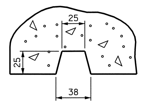
DETAIL "A" (CHAMFER)
