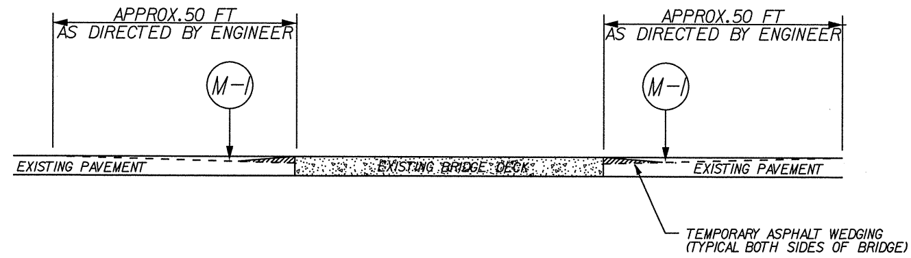
DETAIL NO. 3 MILLING AT BRIDGE APPROACH
