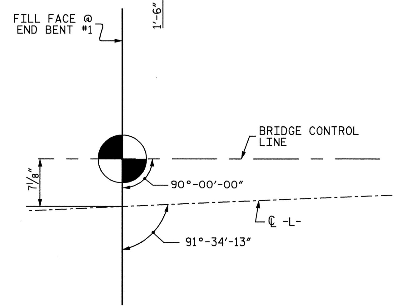
DETAIL "A"
