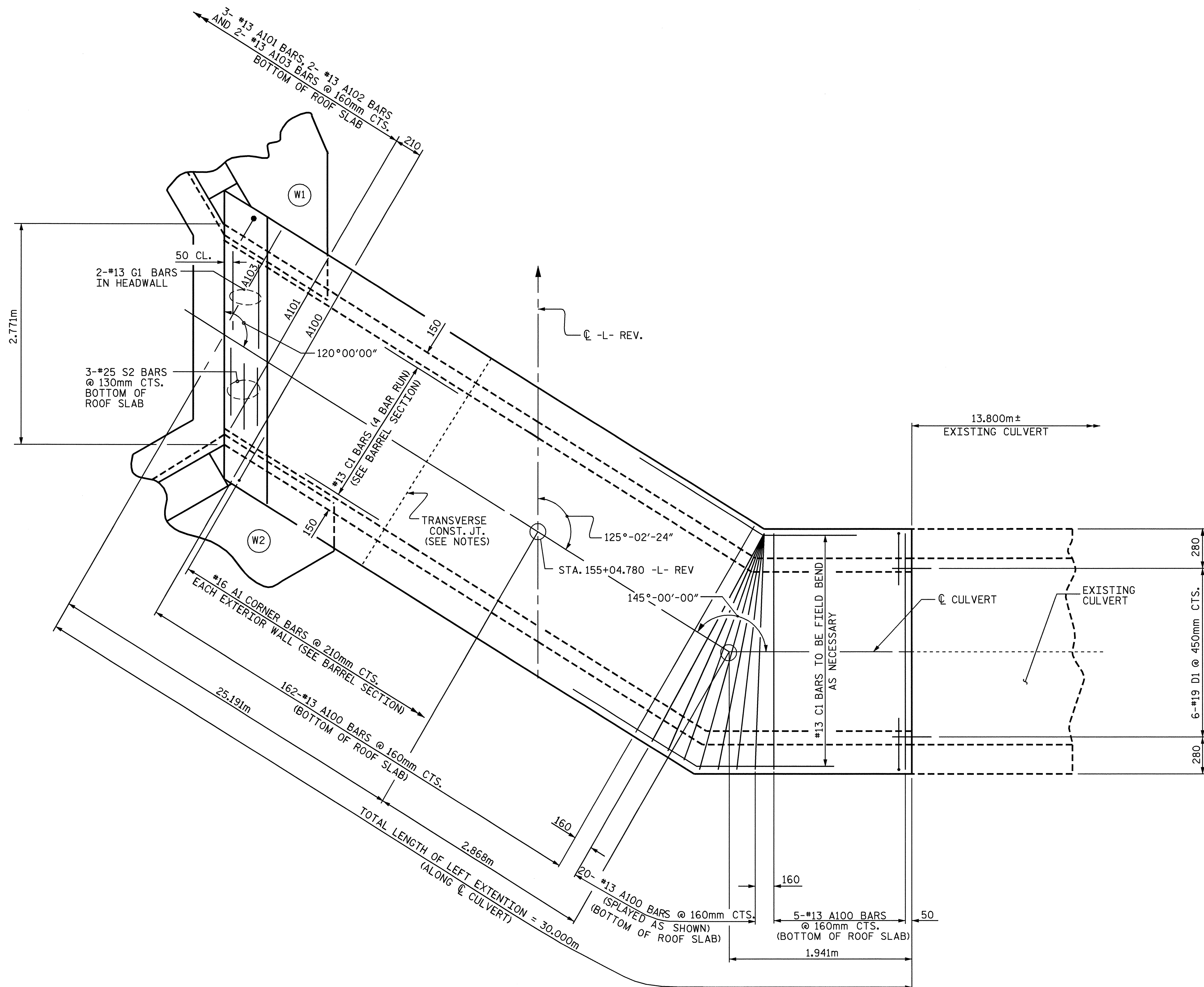
PLAN - ROOF SLAB
