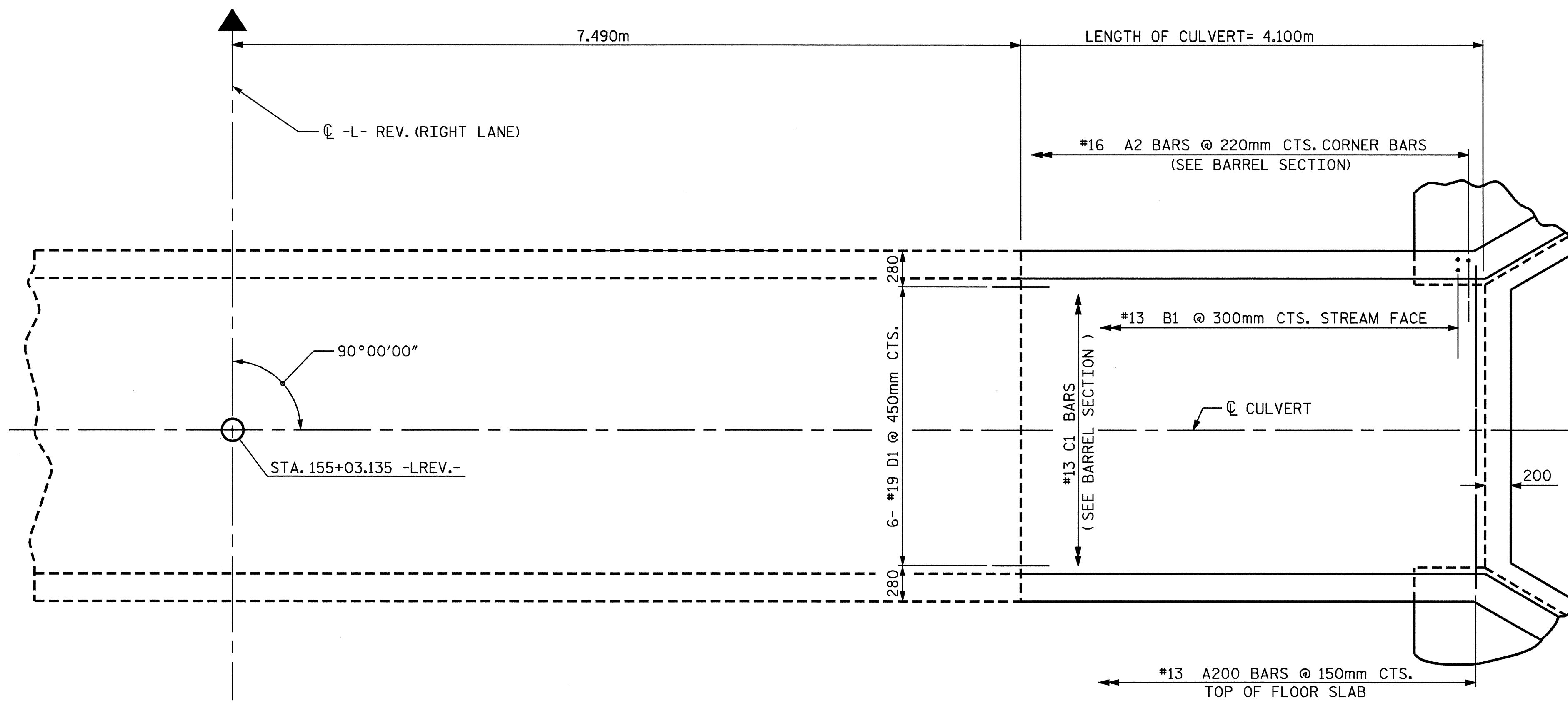
PLAN - ROOF SLAB
