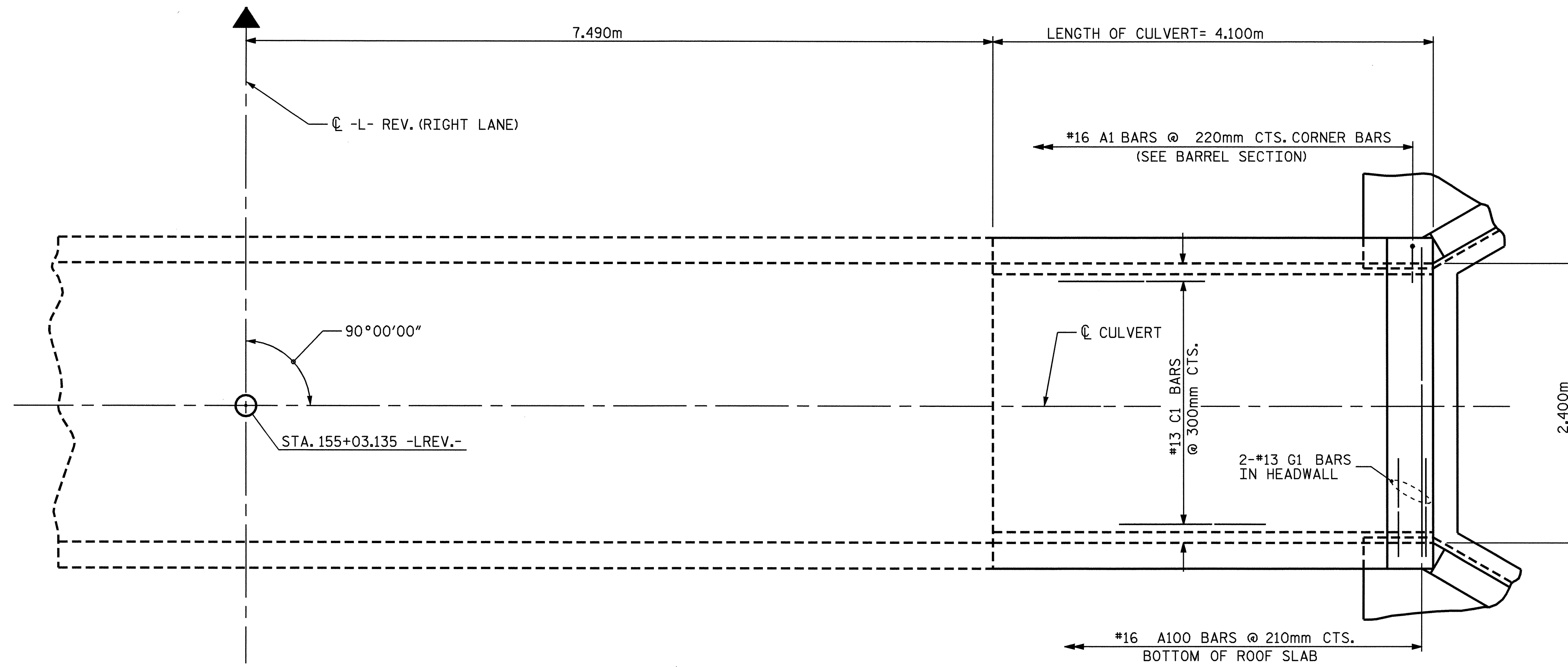
PLAN - ROOF SLAB
