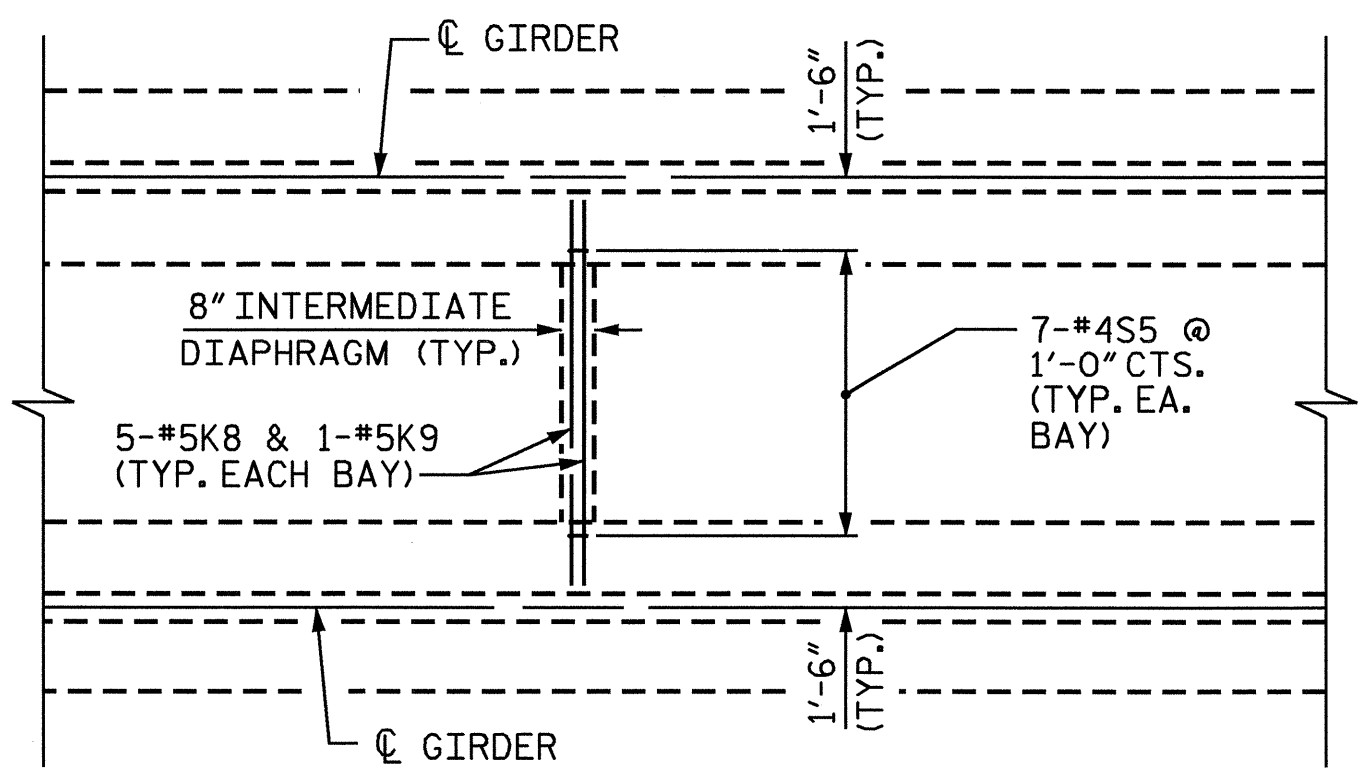
TYPICAL PLAN OF INTERMEDIATE DIAPHRAGM
