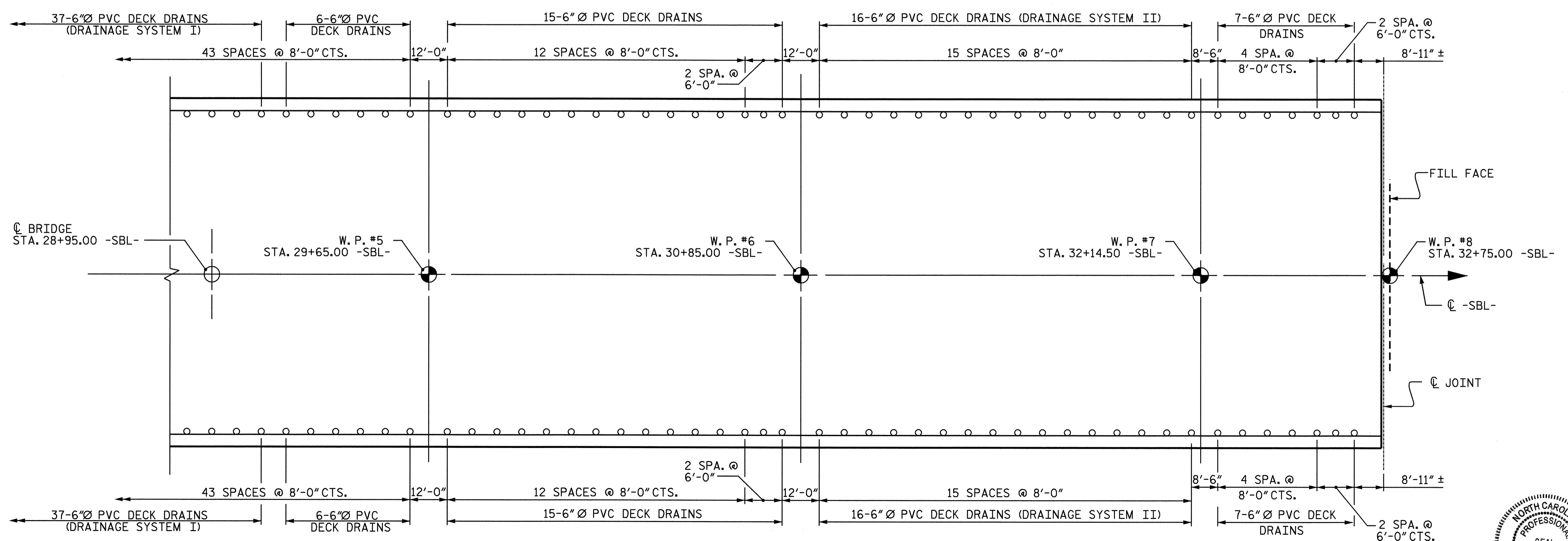
PARTIAL DECK DRAINAGE LAYOUT
