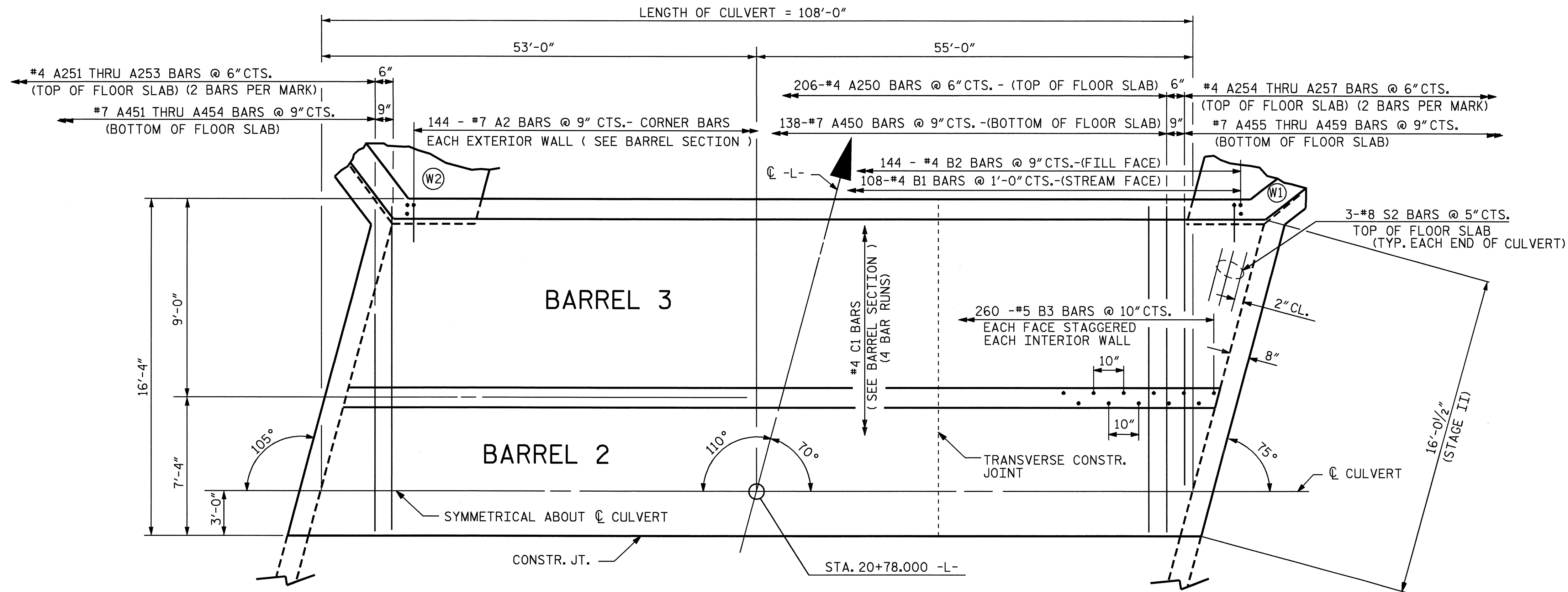
PLAN OF FLOOR SLAB- STAGE II
