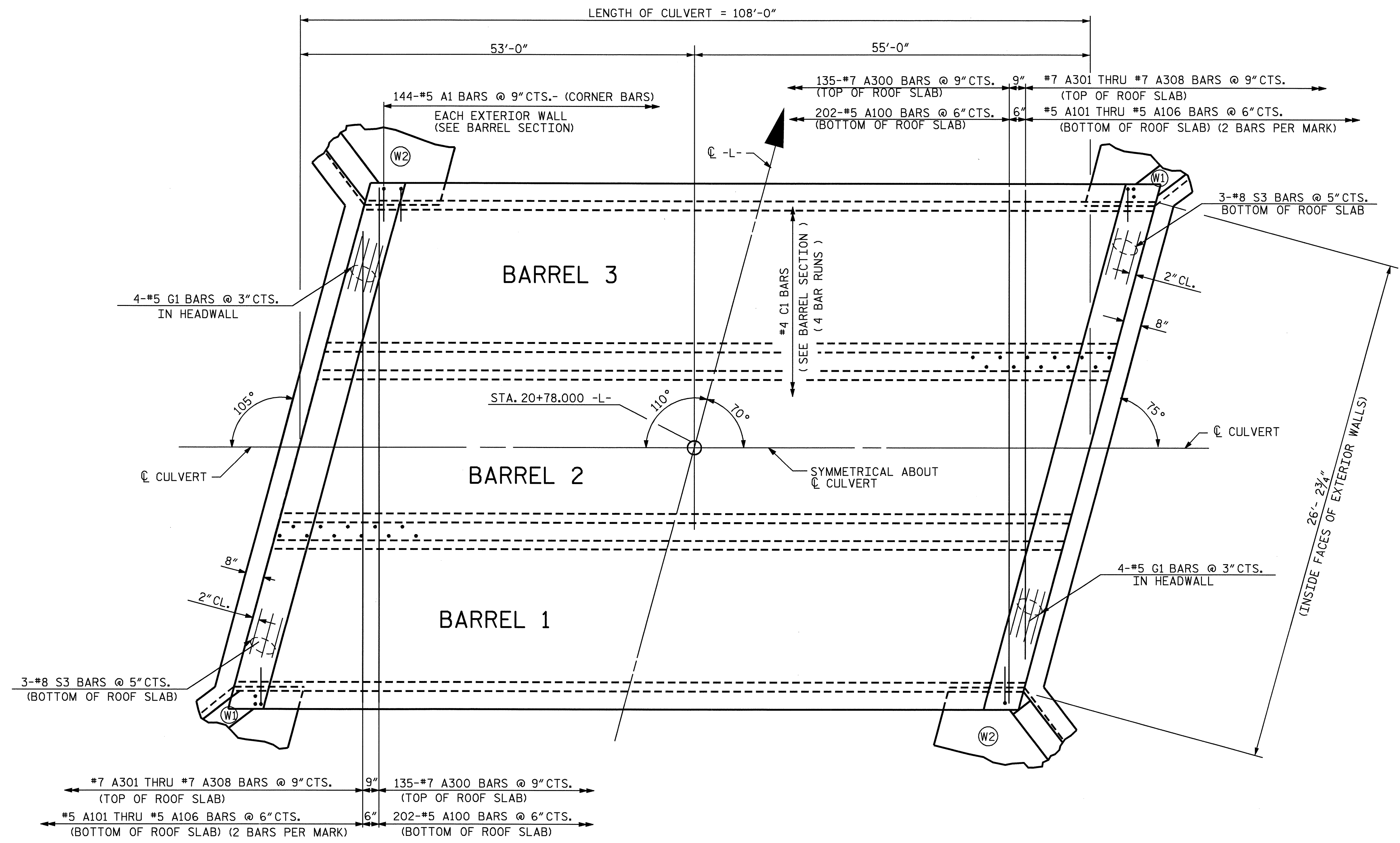
PLAN OF ROOF SLAB- STAGE II
