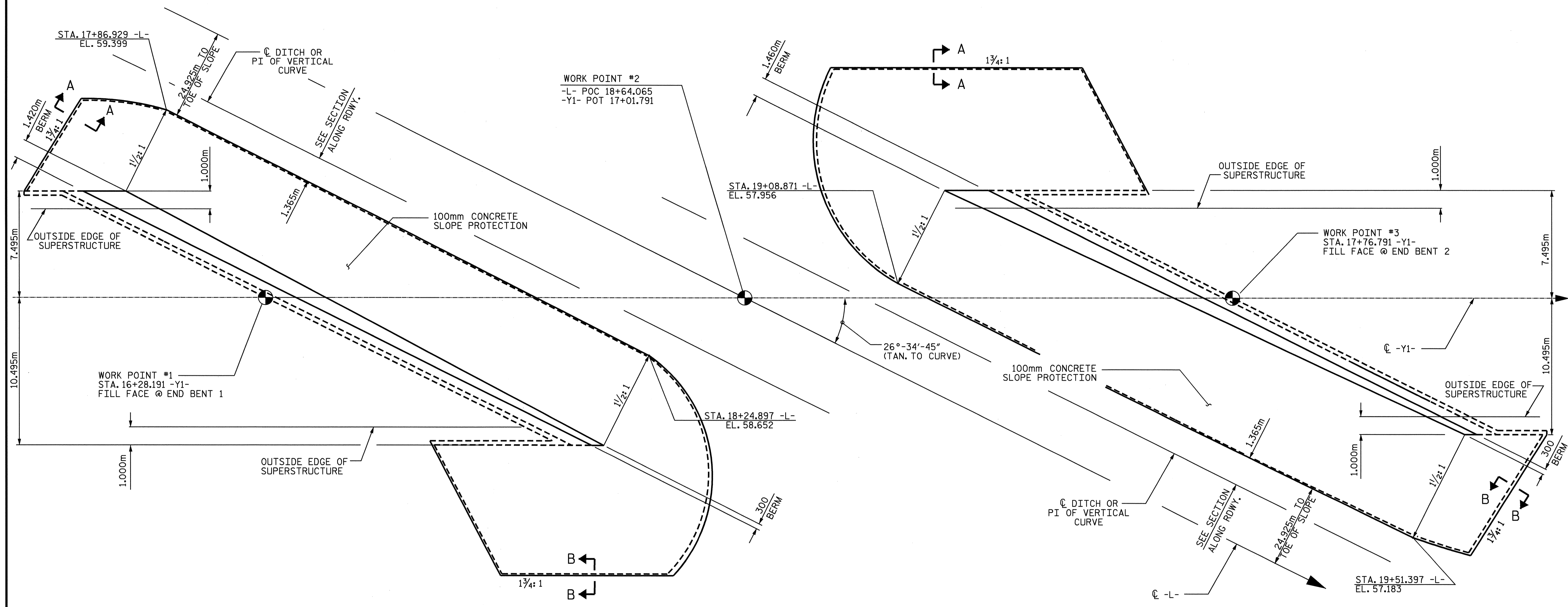
PLAN @ END BENT 1
