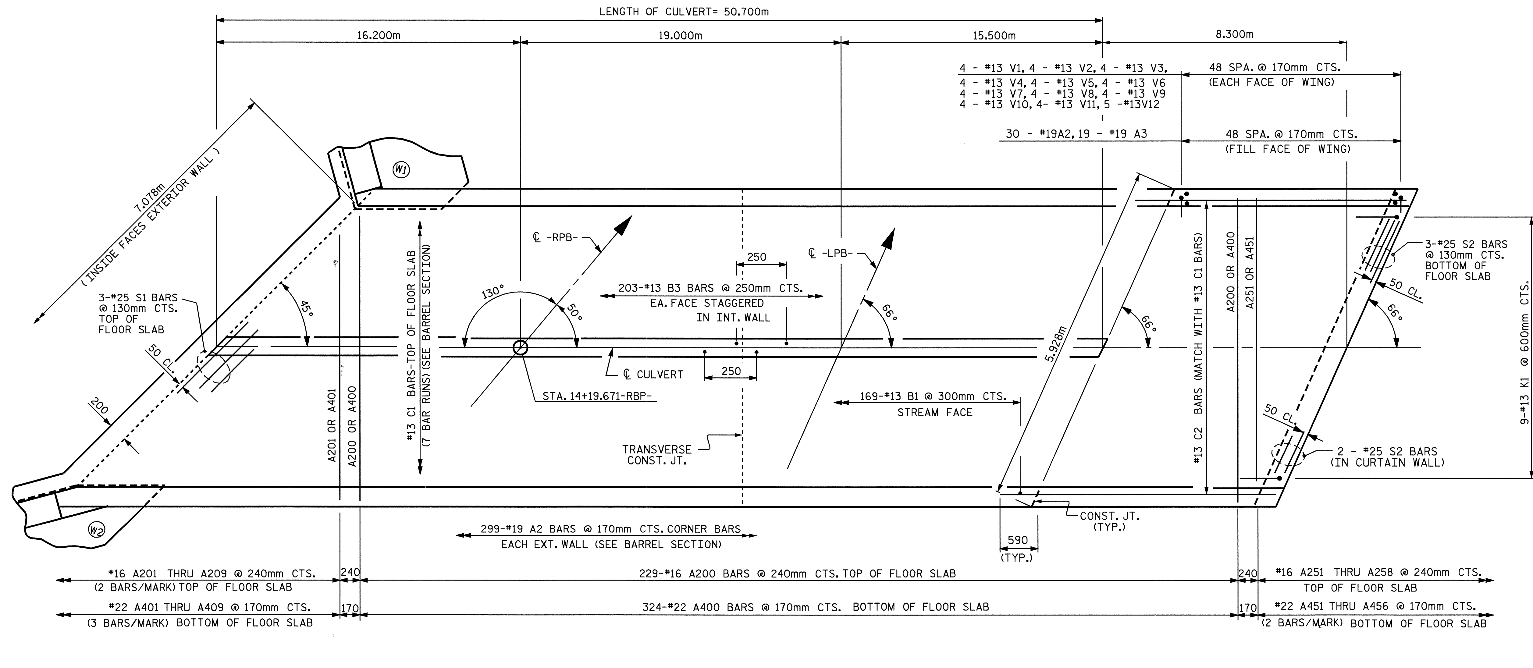
PLAN - FLOOR SLAB
