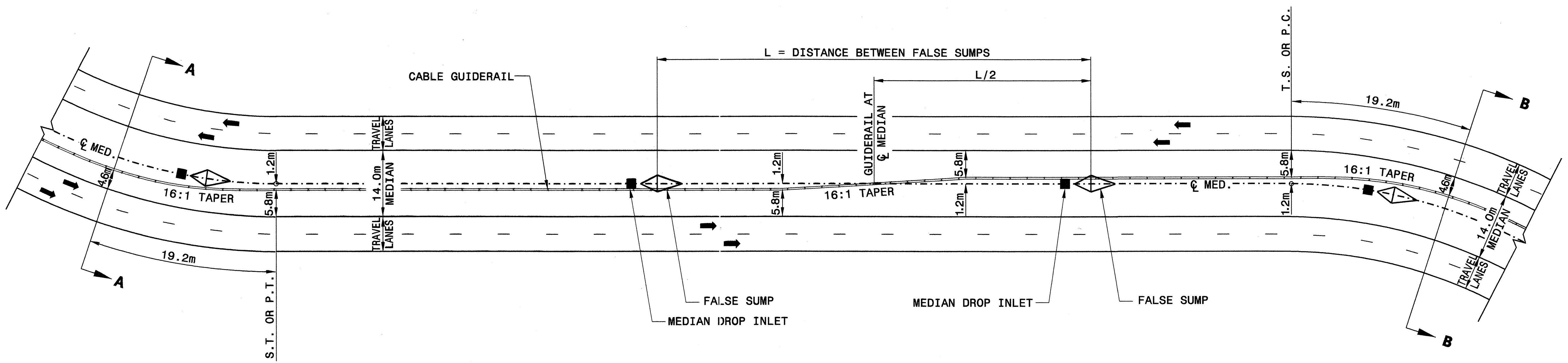
PLAN VIEW
