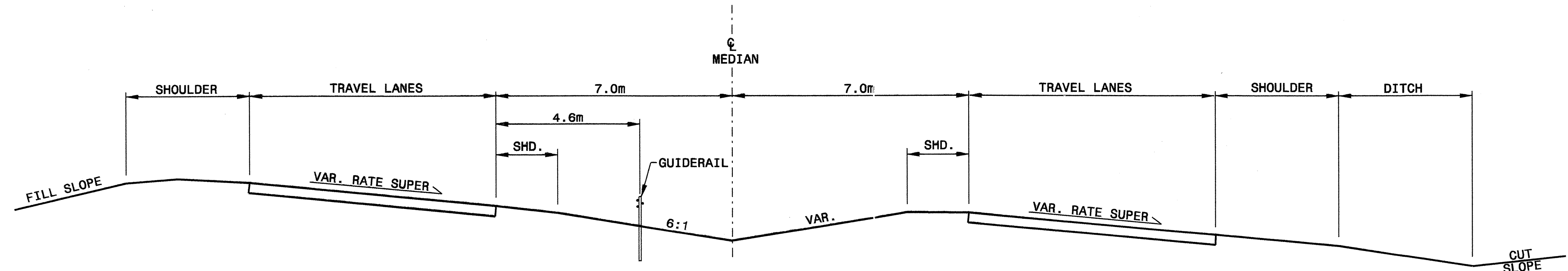
SECTION B-B
