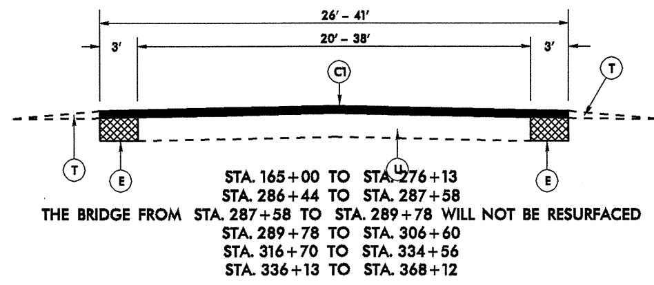
TYPICAL SECTION NO. 1
