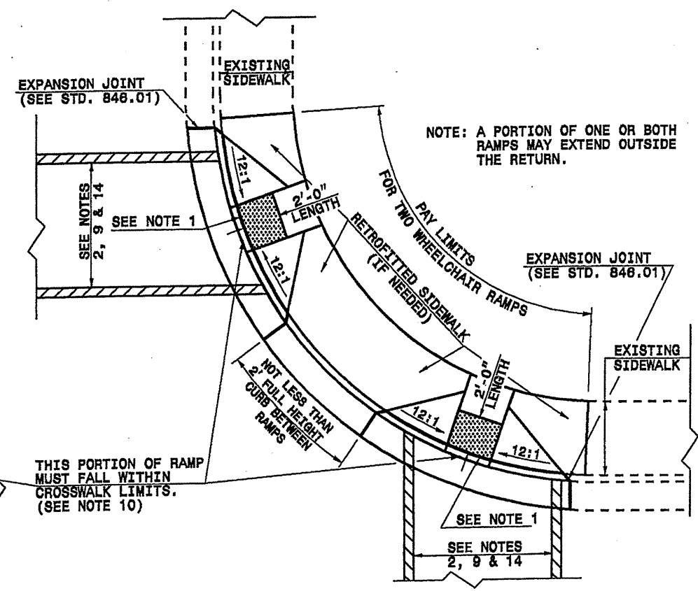
PLAN VIEW DUAL RAMP ANY RADII (40" MIN. FLOOR WIDTH)
