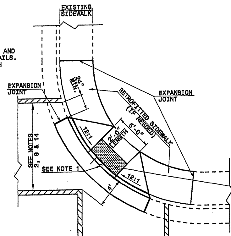
PLAN VIEW DIAGONAL RAMP MAX. 25' RADII (60" MIN. FLOOR WIDTH)
