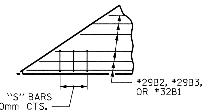
DETAIL A (OPPOSITE END SIMILAR BY ROTATION)
