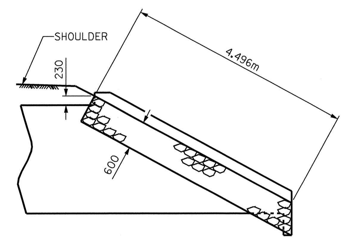
ELEVATION VIEW
