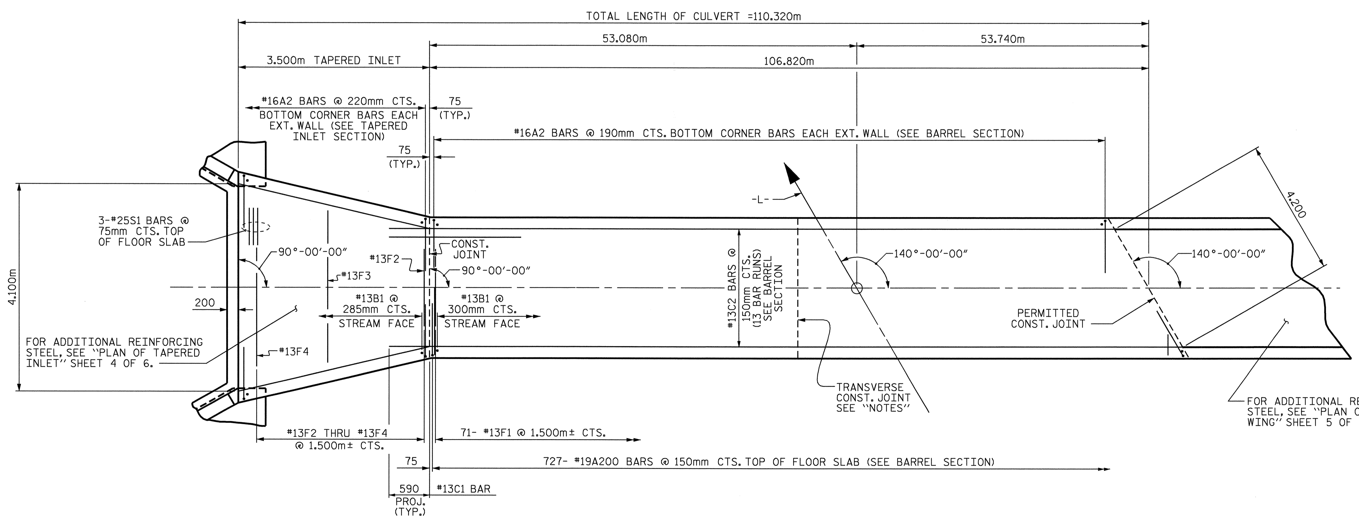
PLAN OF FLOOR SLAB
