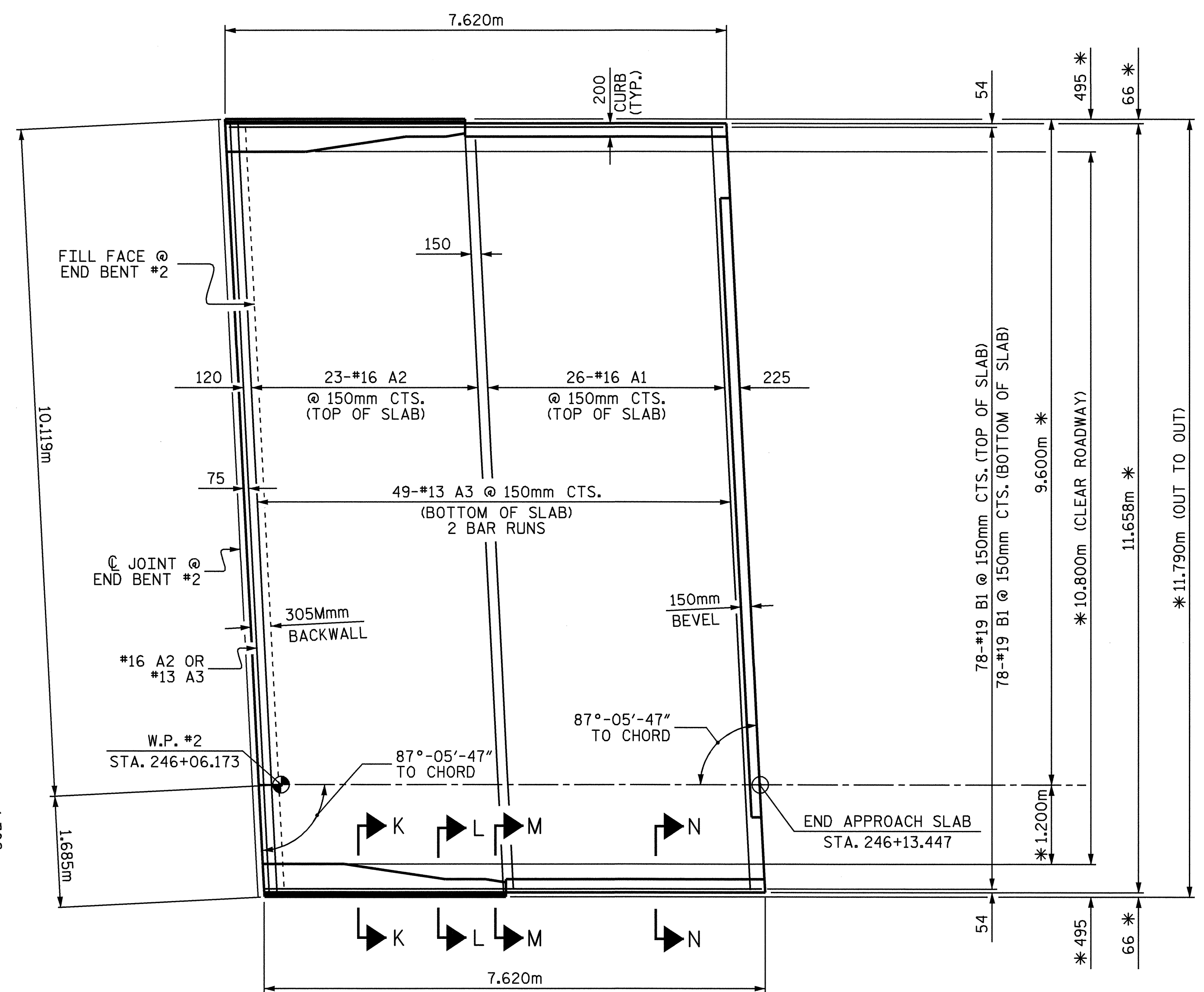
PLAN @ END BENT #2
