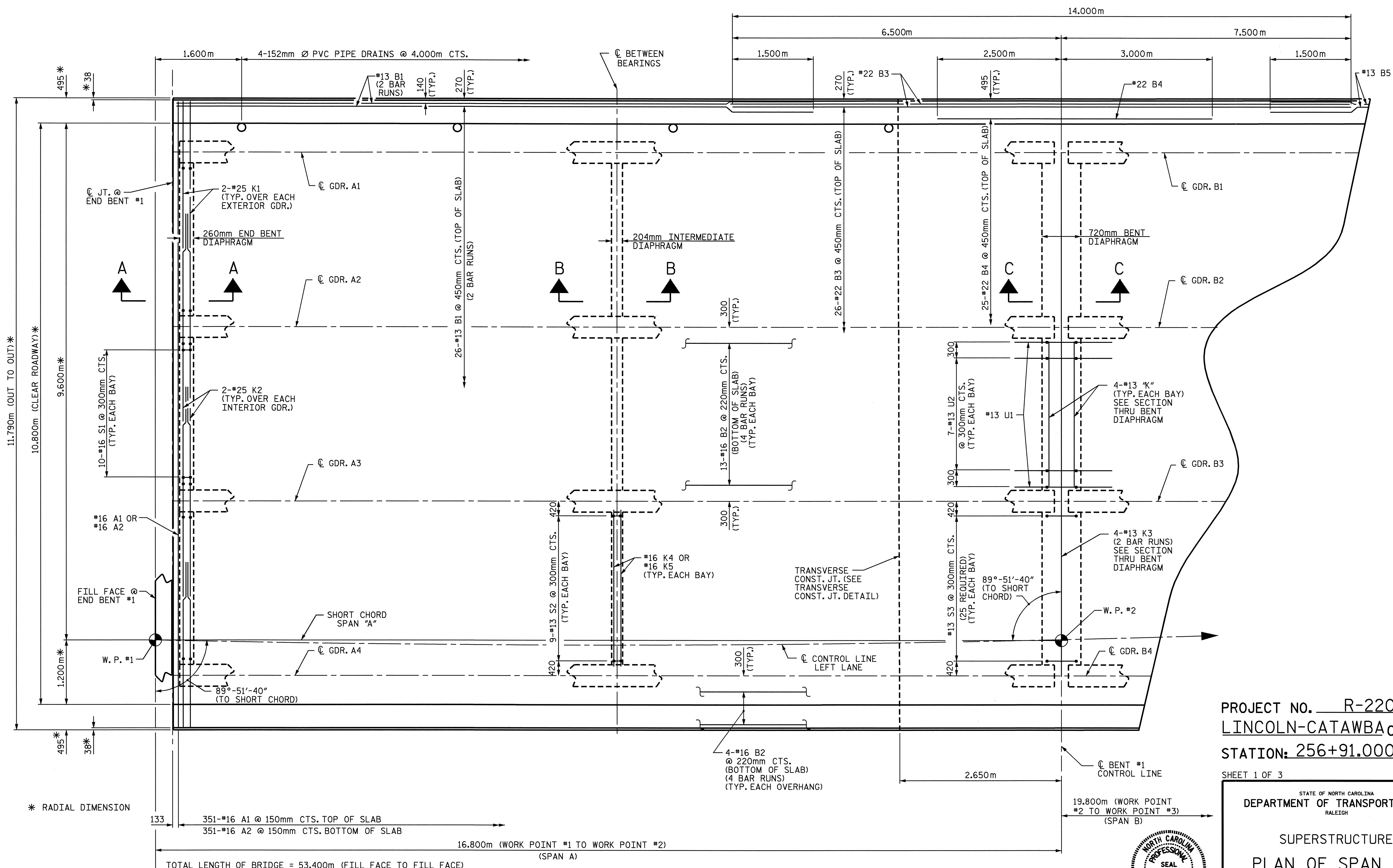
PLAN OF SPAN "A" ARC OFFSETS ON SPAN "A" ARE NEGLIGIBLE.
