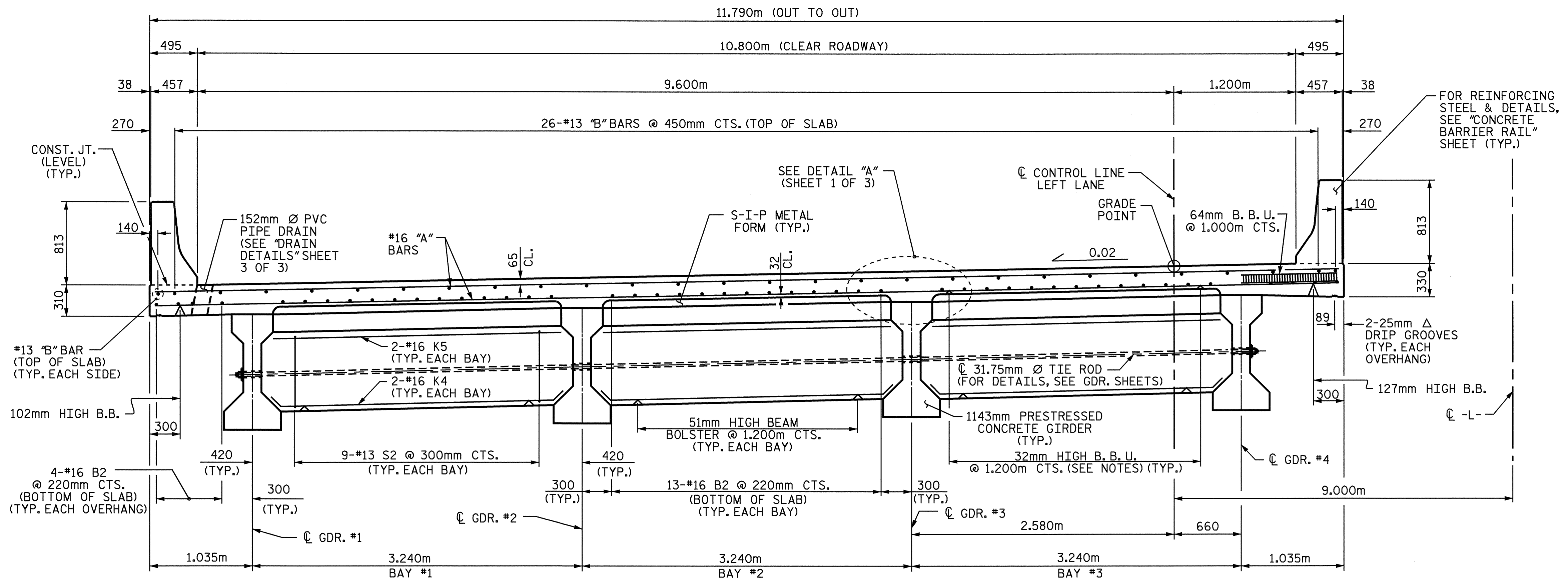
TYPICAL SECTION @ INTERMEDIATE DIAPHRAGM
