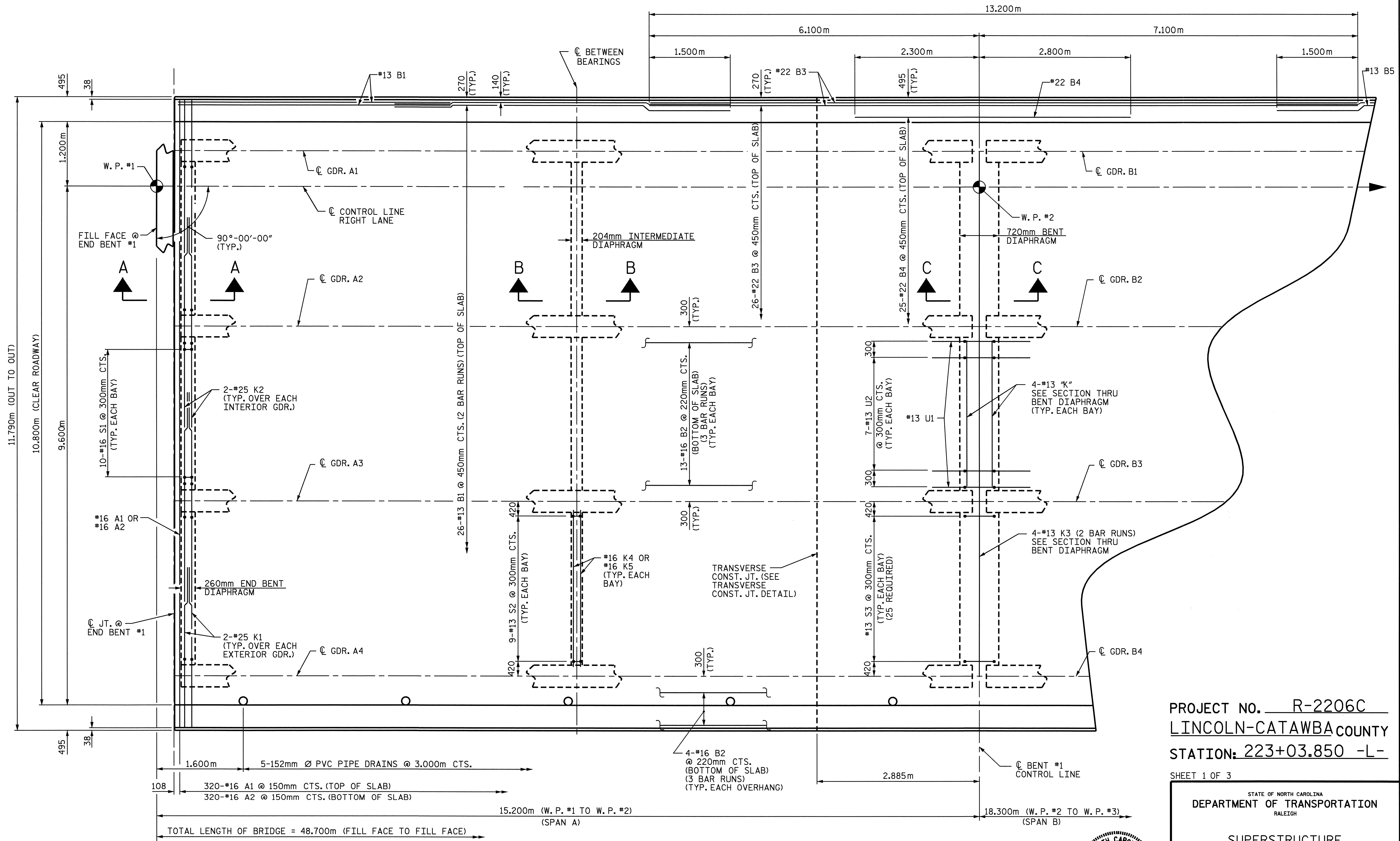
PLAN OF SPAN "A"
