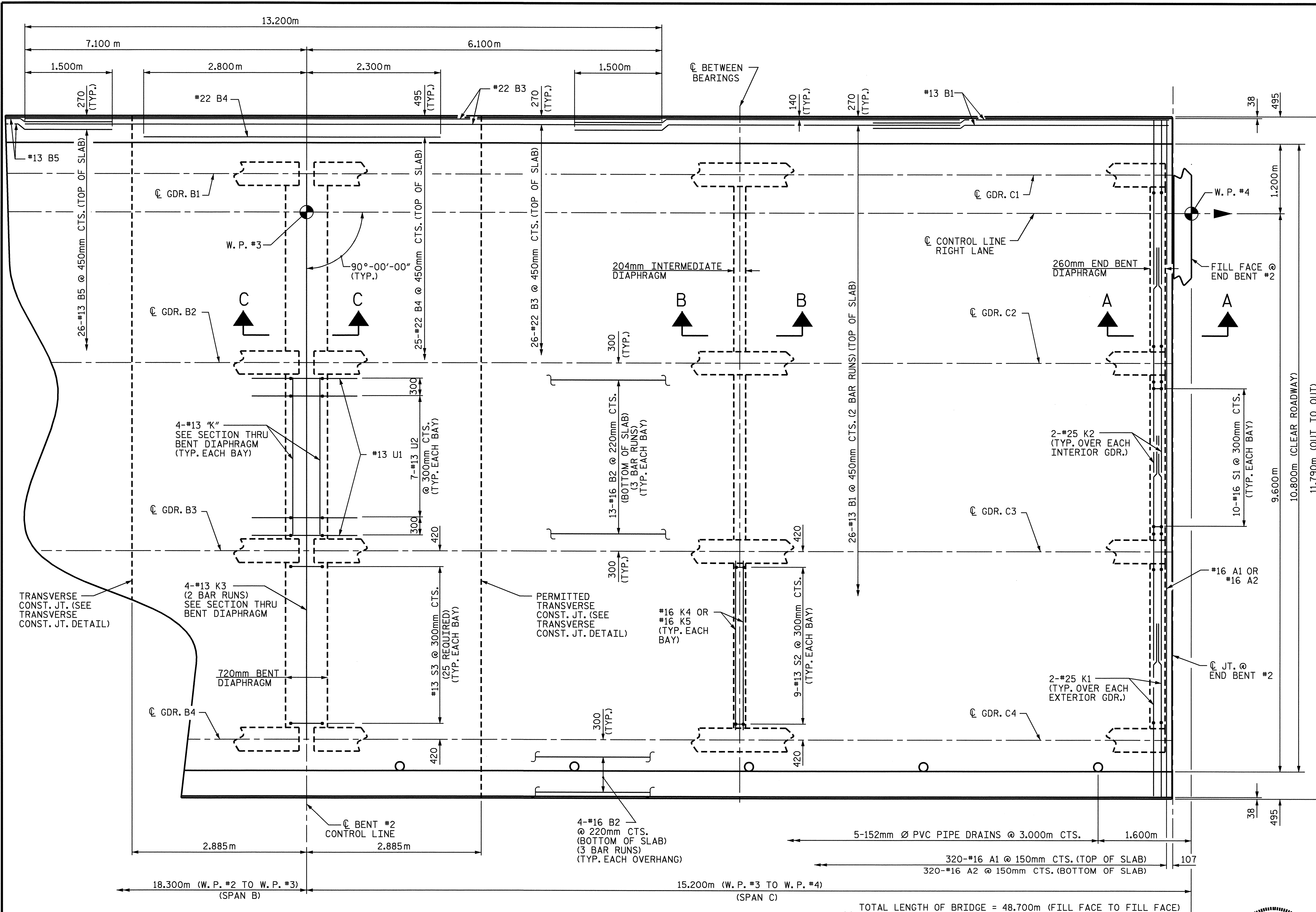
PLAN OF SPAN "C"
