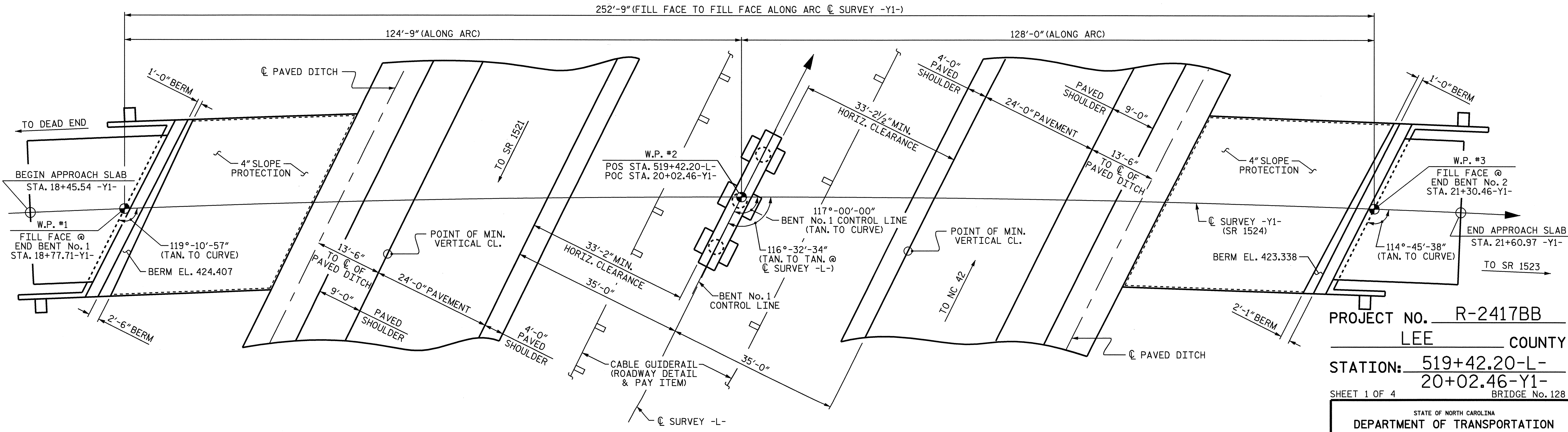
PLAN (PILES FOR END BENTS AND BENTS NOT SHOWN FOR CLARITY)
