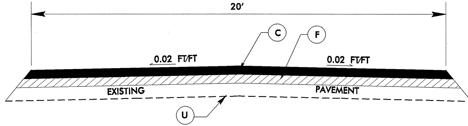
TYPICAL SECTION NO. 7
