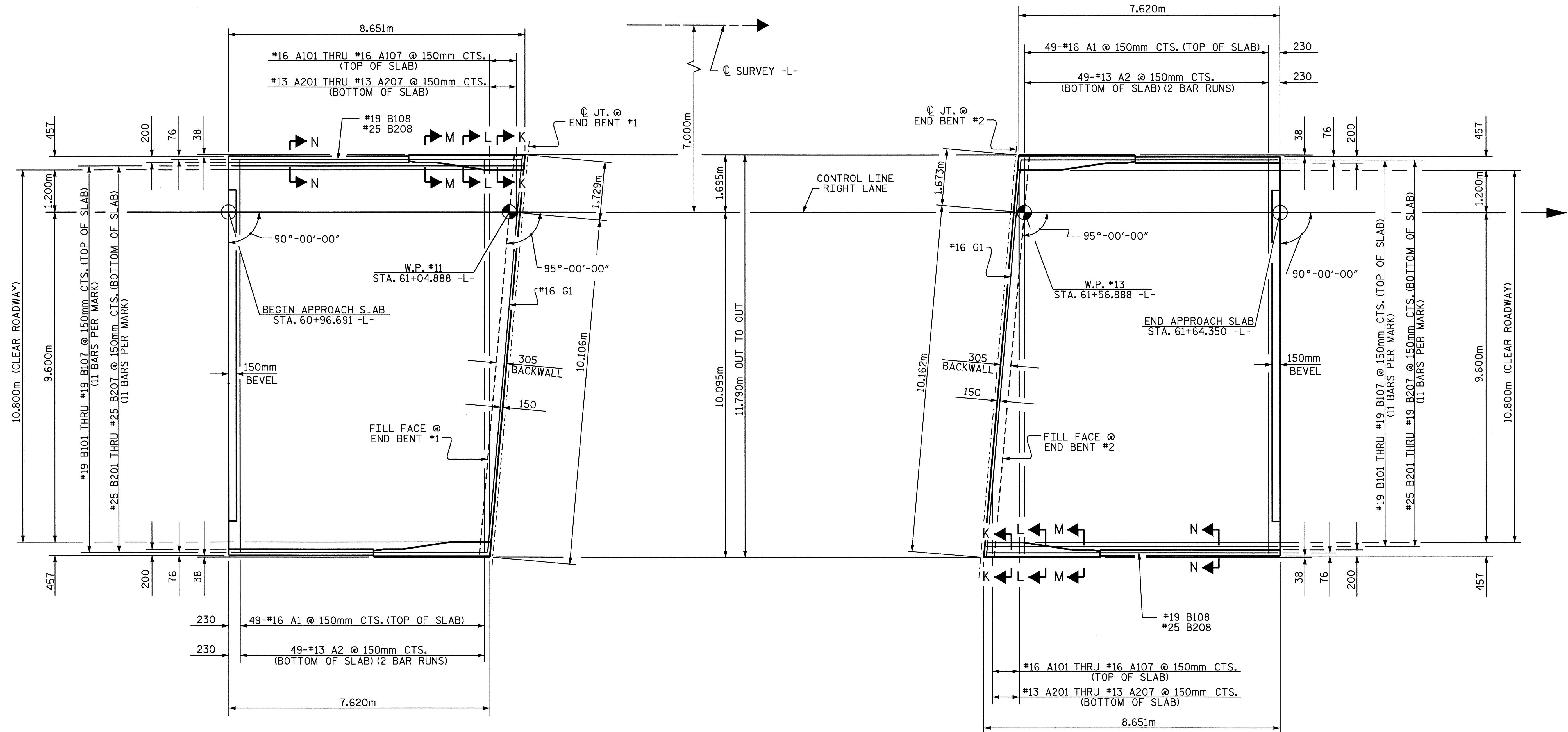
PLAN OF APPROACH SLAB @ END BENT #1
