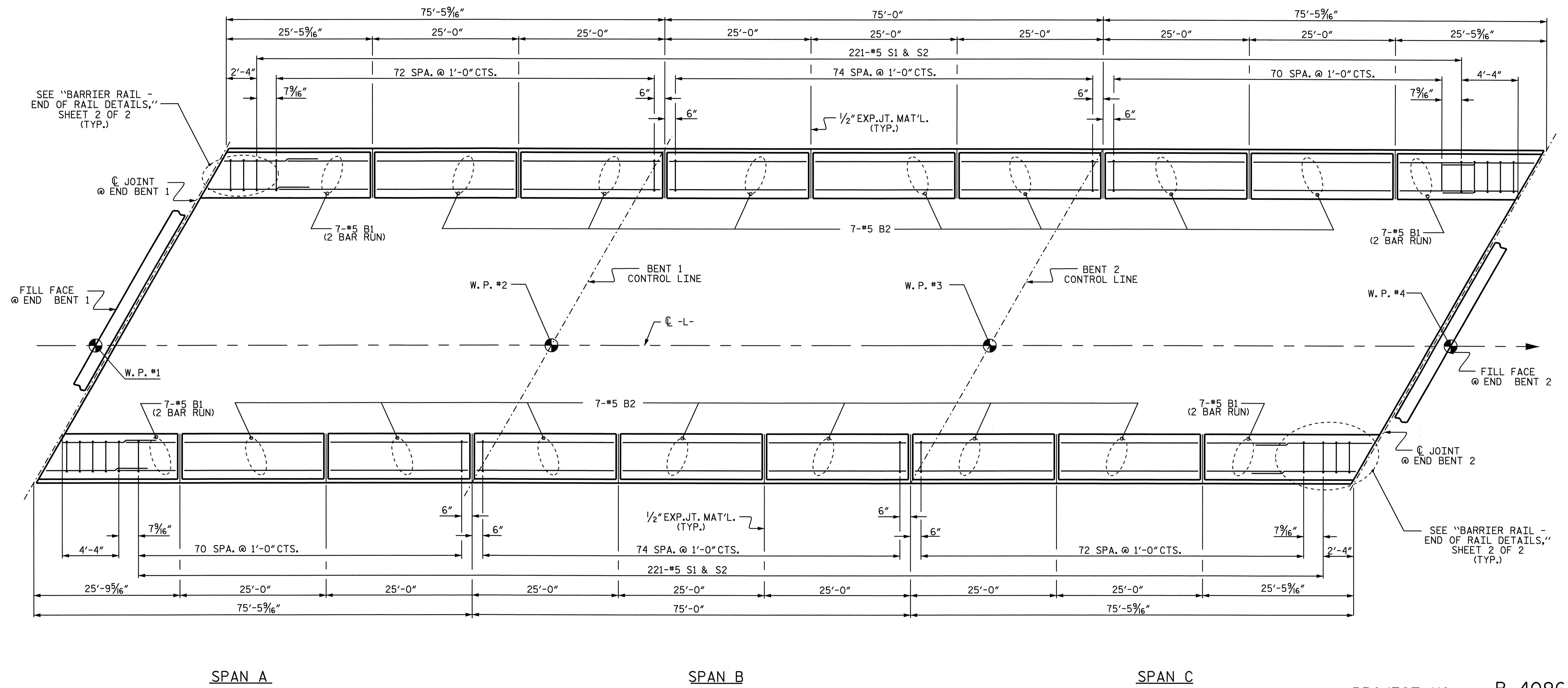
PLAN
