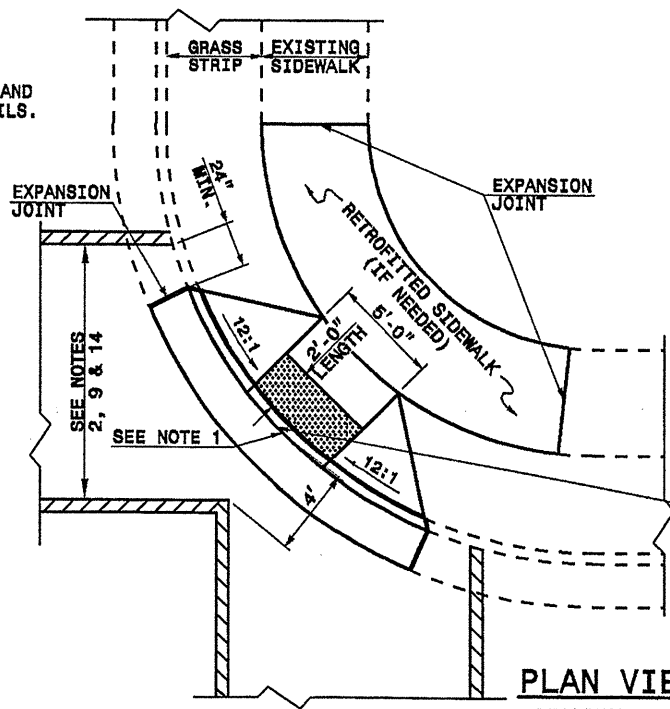
DETECTABLE WARNING DOMES
