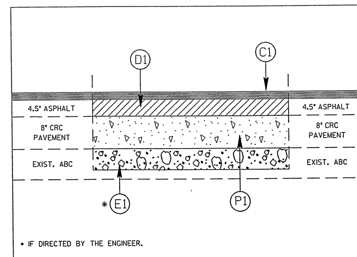
PATCHING TYPICAL
