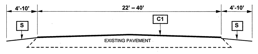
TYPICAL SECTION NO. 1 NOTE: INCLUDES MILLING AT BRIDGE APPROACHES
