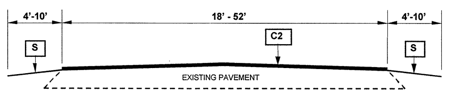
TYPICAL SECTION NO. 2 NOTE: INCLUDES MILLING AT BRIDGE APPROACHES
