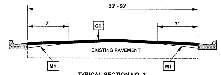
TYPICAL SECTION NO. 3
