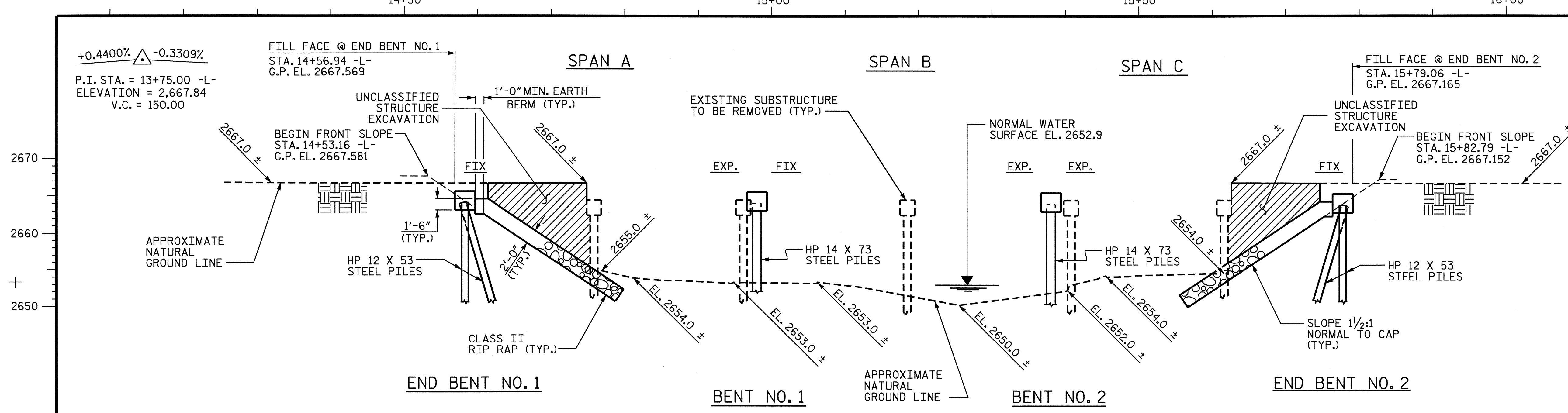
SECTION ALONG C SURVEY -L-
