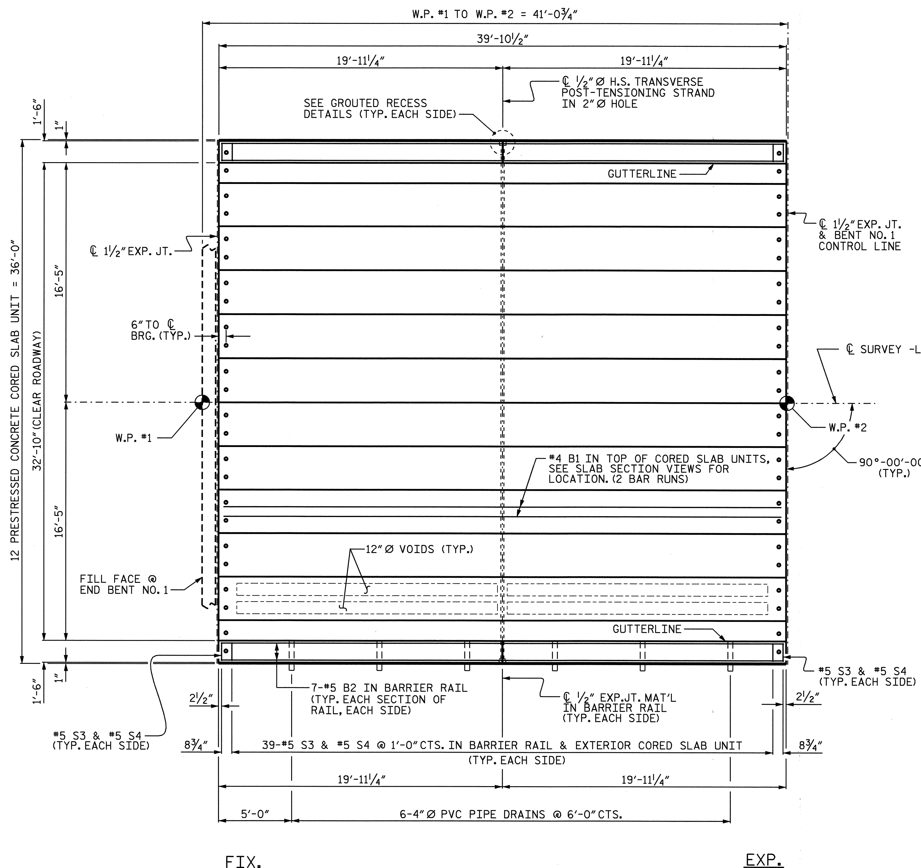
PLAN OF SPAN "A"
