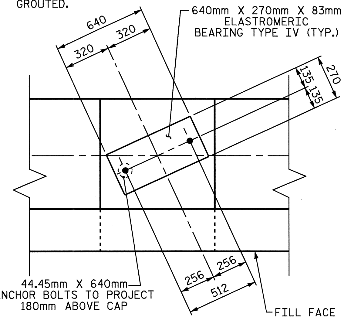
DETAIL A
