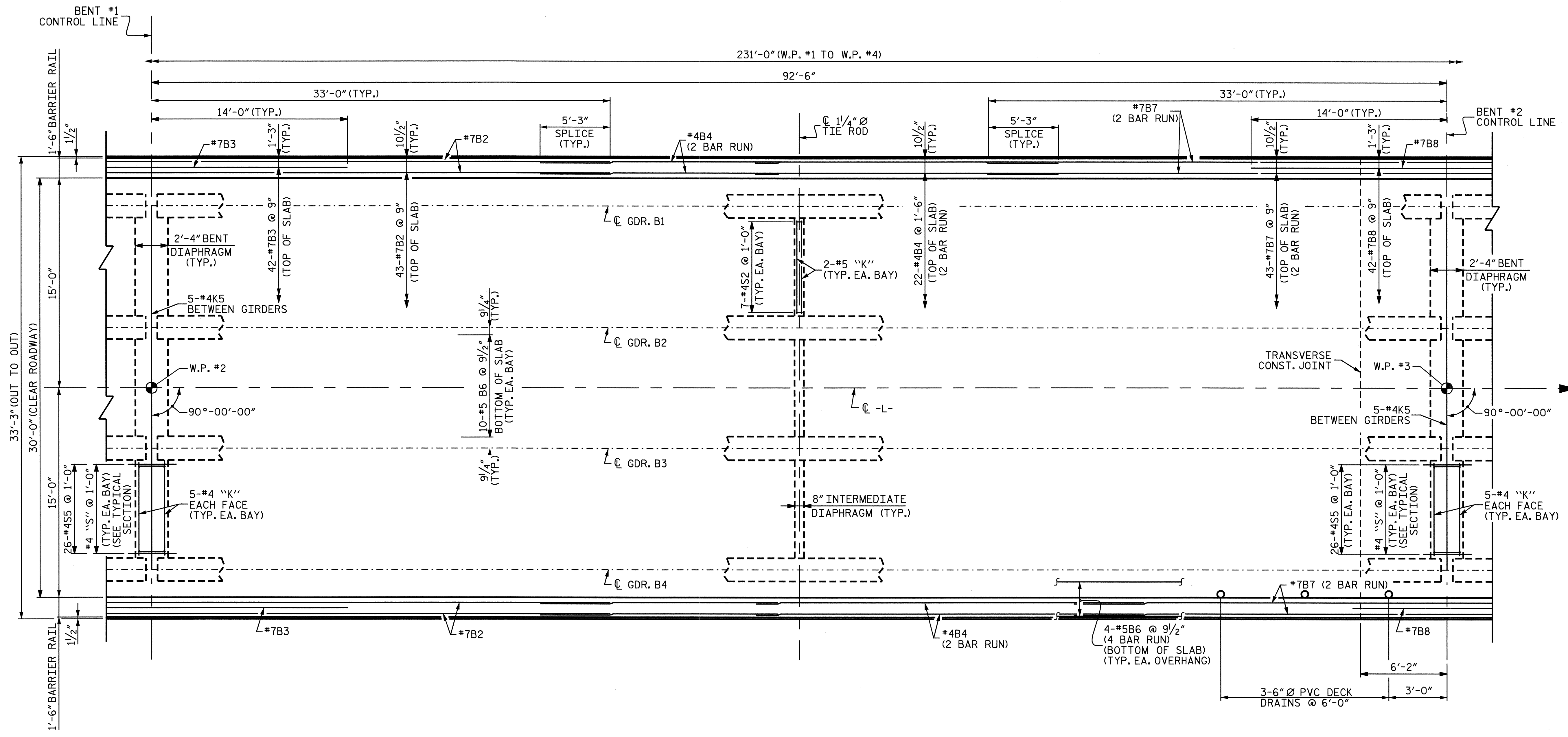
PLAN OF SPAN B
