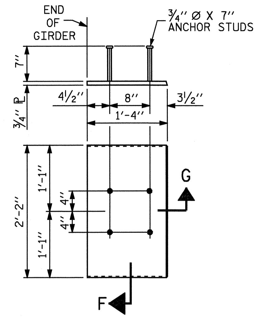
DETAIL "A" (FOR AASHTO TYPE IV GIRDERS)
