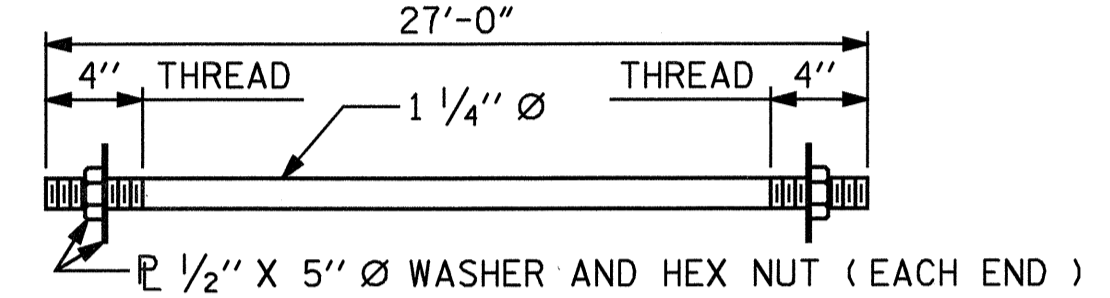
1 1/4" Ø TIE ROD ASSEMBLY (3 COMPLETE ASSEMBLIES REQUIRED)
