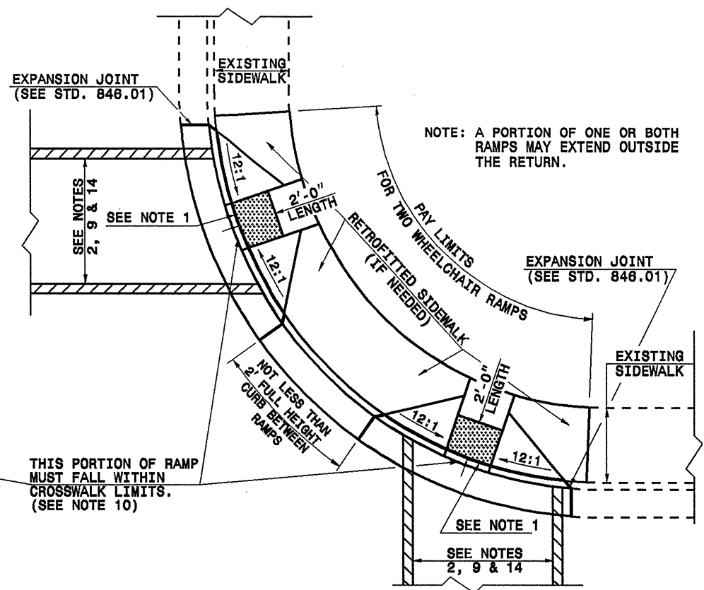
PLAN VIEW
